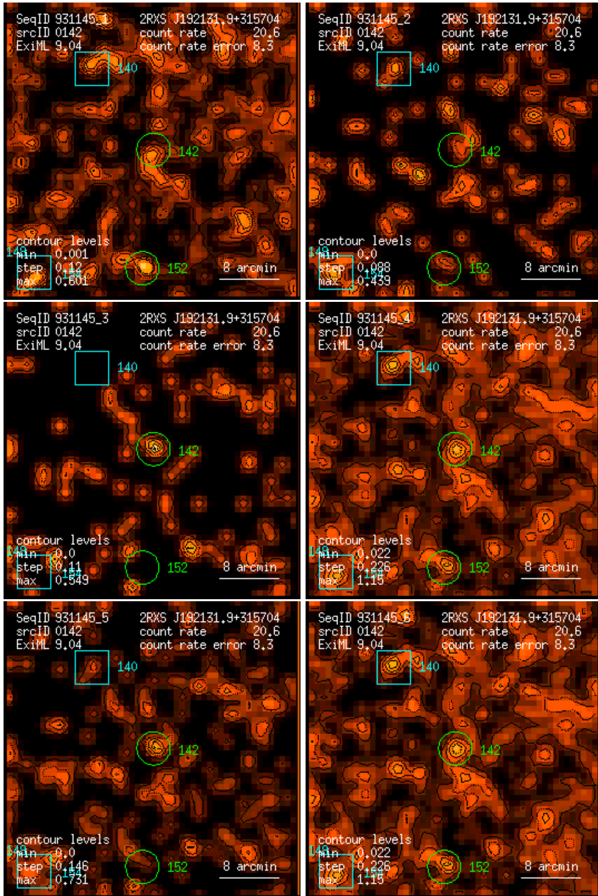
Figure 142: RASS 931145: detection 0142: band rate images, Gaussian filter: (1) PSPC channels 11 – 41, (2) 52 – 90, (3) 91 – 201, (4) 11 – 235, (5) 52 – 201, (6) 11 – 201. Broad band rates in counts/ks. Band rate contour levels in counts/ks/arcmin 2 .
