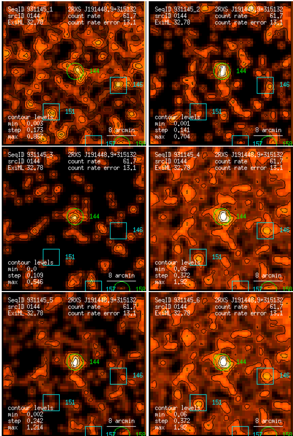
Figure 144: RASS 931145: detection 0144: band rate images, Gaussian filter: (1) PSPC channels 11 – 41, (2) 52 – 90, (3) 91 – 201, (4) 11 – 235, (5) 52 – 201, (6) 11 – 201. Broad band rates in counts/ks. Band rate contour levels in counts/ks/arcmin 2 .
