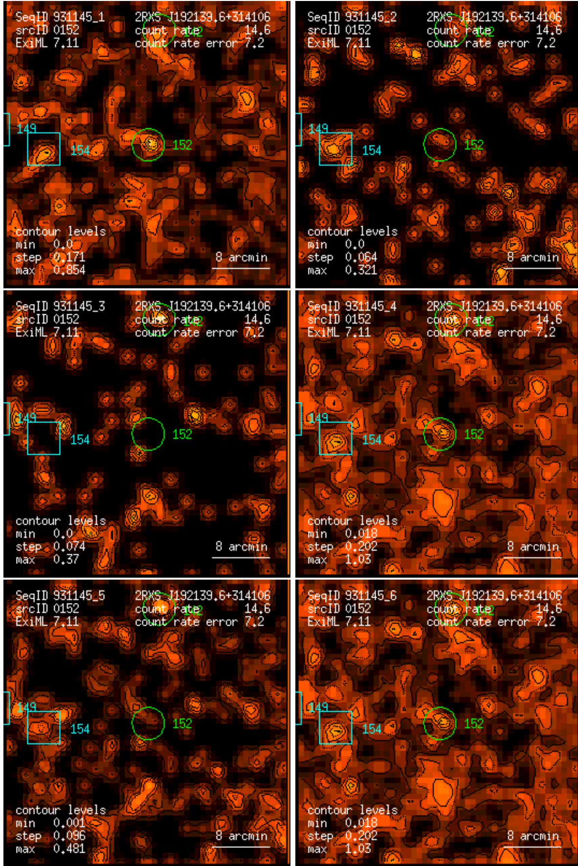
Figure 152: RASS 931145: detection 0152: band rate images, Gaussian filter: (1) PSPC channels 11 – 41, (2) 52 – 90, (3) 91 – 201, (4) 11 – 235, (5) 52 – 201, (6) 11 – 201. Broad band rates in counts/ks. Band rate contour levels in counts/ks/arcmin 2 .
