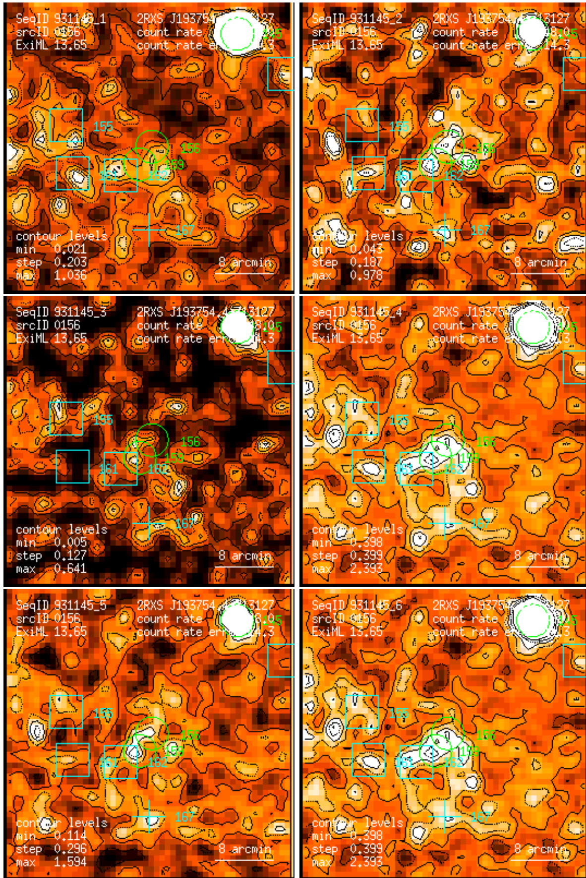
Figure 156: RASS 931145: detection 0156: band rate images, Gaussian filter: (1) PSPC channels 11 – 41, (2) 52 – 90, (3) 91 – 201, (4) 11 – 235, (5) 52 – 201, (6) 11 – 201. Broad band rates in counts/ks. Band rate contour levels in counts/ks/arcmin 2 .
