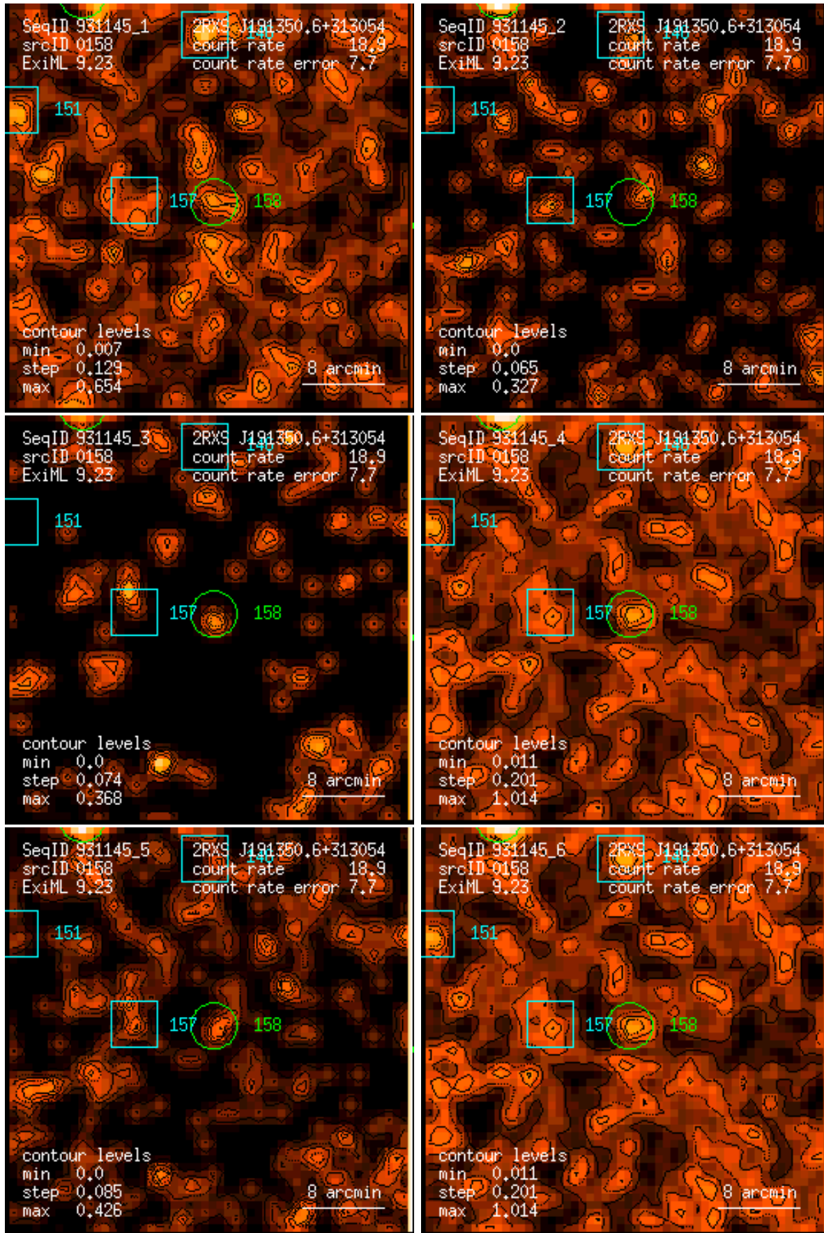
Figure 158: RASS 931145: detection 0158: band rate images, Gaussian filter: (1) PSPC channels 11 – 41, (2) 52 – 90, (3) 91 – 201, (4) 11 – 235, (5) 52 – 201, (6) 11 – 201. Broad band rates in counts/ks. Band rate contour levels in counts/ks/arcmin 2 .
