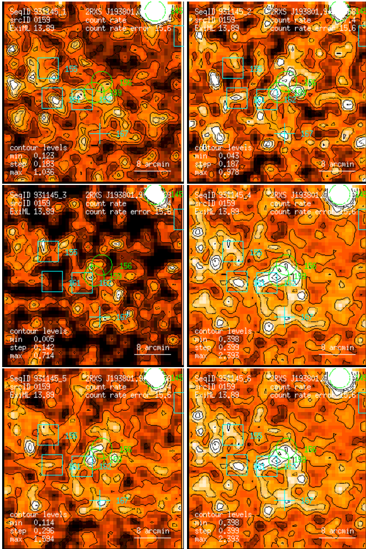
Figure 159: RASS 931145: detection 0159: band rate images, Gaussian filter: (1) PSPC channels 11 – 41, (2) 52 – 90, (3) 91 – 201, (4) 11 – 235, (5) 52 – 201, (6) 11 – 201. Broad band rates in counts/ks. Band rate contour levels in counts/ks/arcmin 2 .
