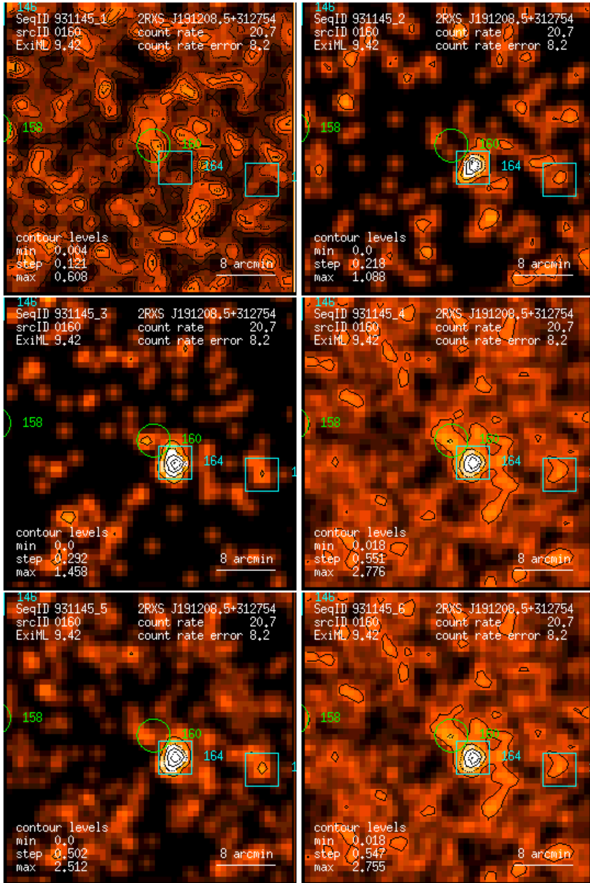
Figure 160: RASS 931145: detection 0160: band rate images, Gaussian filter: (1) PSPC channels 11 – 41, (2) 52 – 90, (3) 91 – 201, (4) 11 – 235, (5) 52 – 201, (6) 11 – 201. Broad band rates in counts/ks. Band rate contour levels in counts/ks/arcmin 2 .
