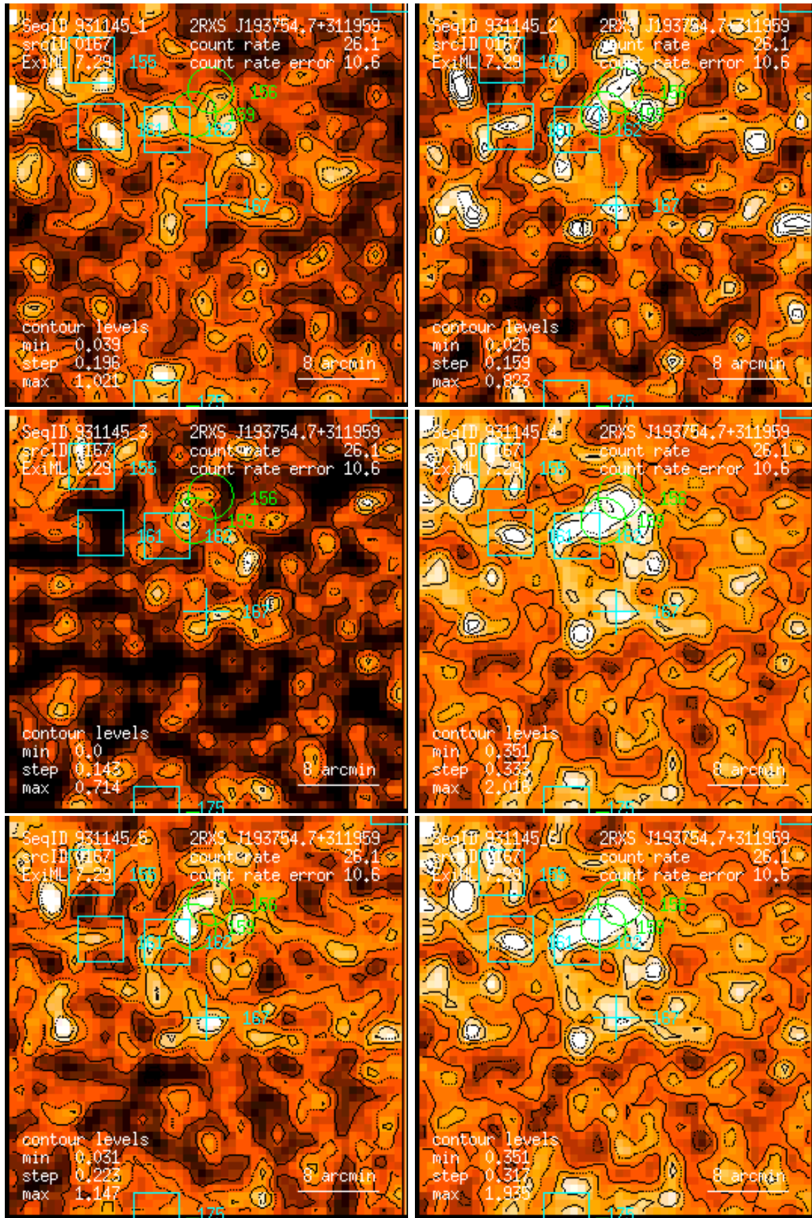
Figure 167: RASS 931145: detection 0167: band rate images, Gaussian filter: (1) PSPC channels 11 – 41, (2) 52 – 90, (3) 91 – 201, (4) 11 – 235, (5) 52 – 201, (6) 11 – 201. Broad band rates in counts/ks. Band rate contour levels in counts/ks/arcmin 2 .
