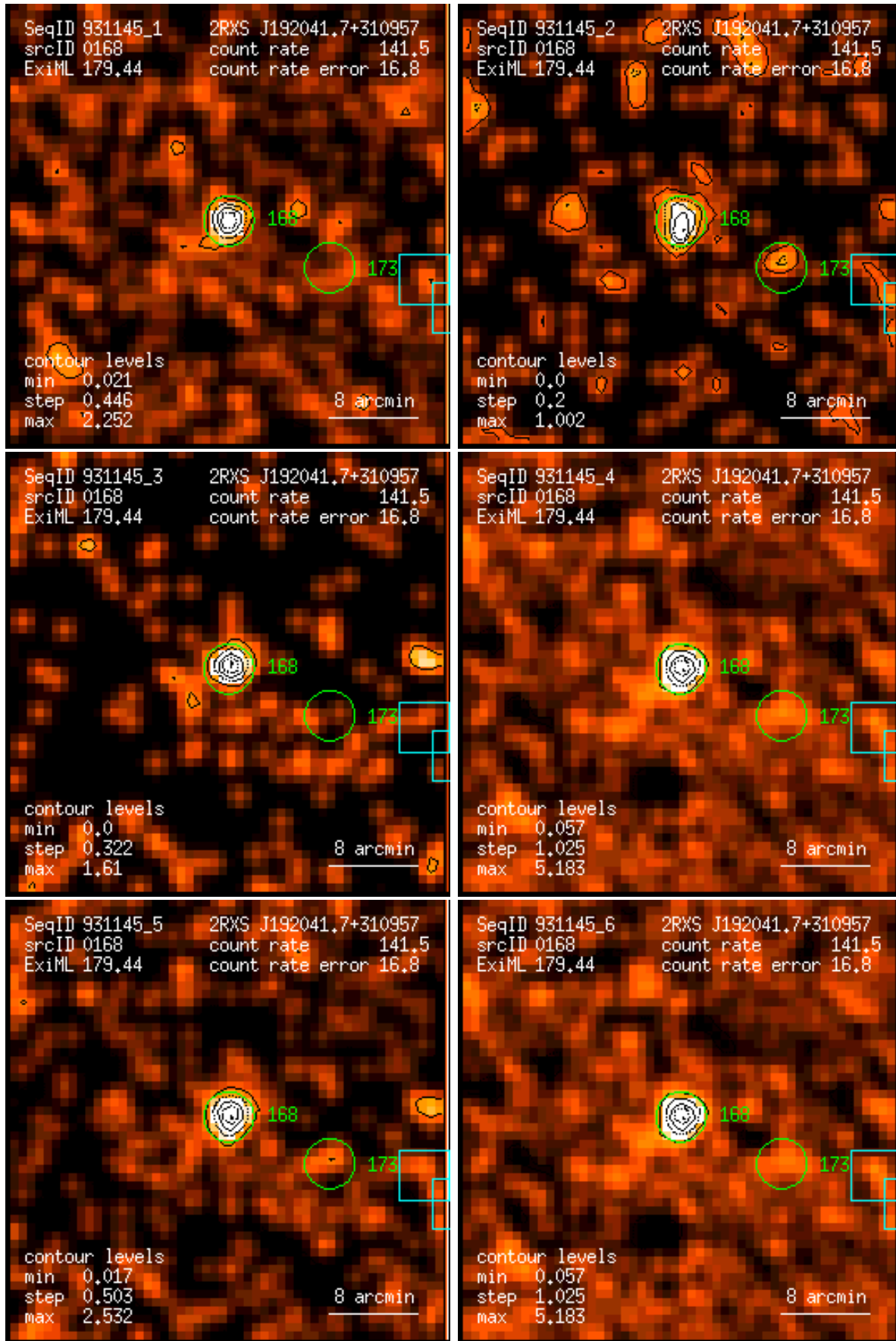
Figure 168: RASS 931145: detection 0168: band rate images, Gaussian filter: (1) PSPC channels 11 – 41, (2) 52 – 90, (3) 91 – 201, (4) 11 – 235, (5) 52 – 201, (6) 11 – 201. Broad band rates in counts/ks. Band rate contour levels in counts/ks/arcmin 2 .
