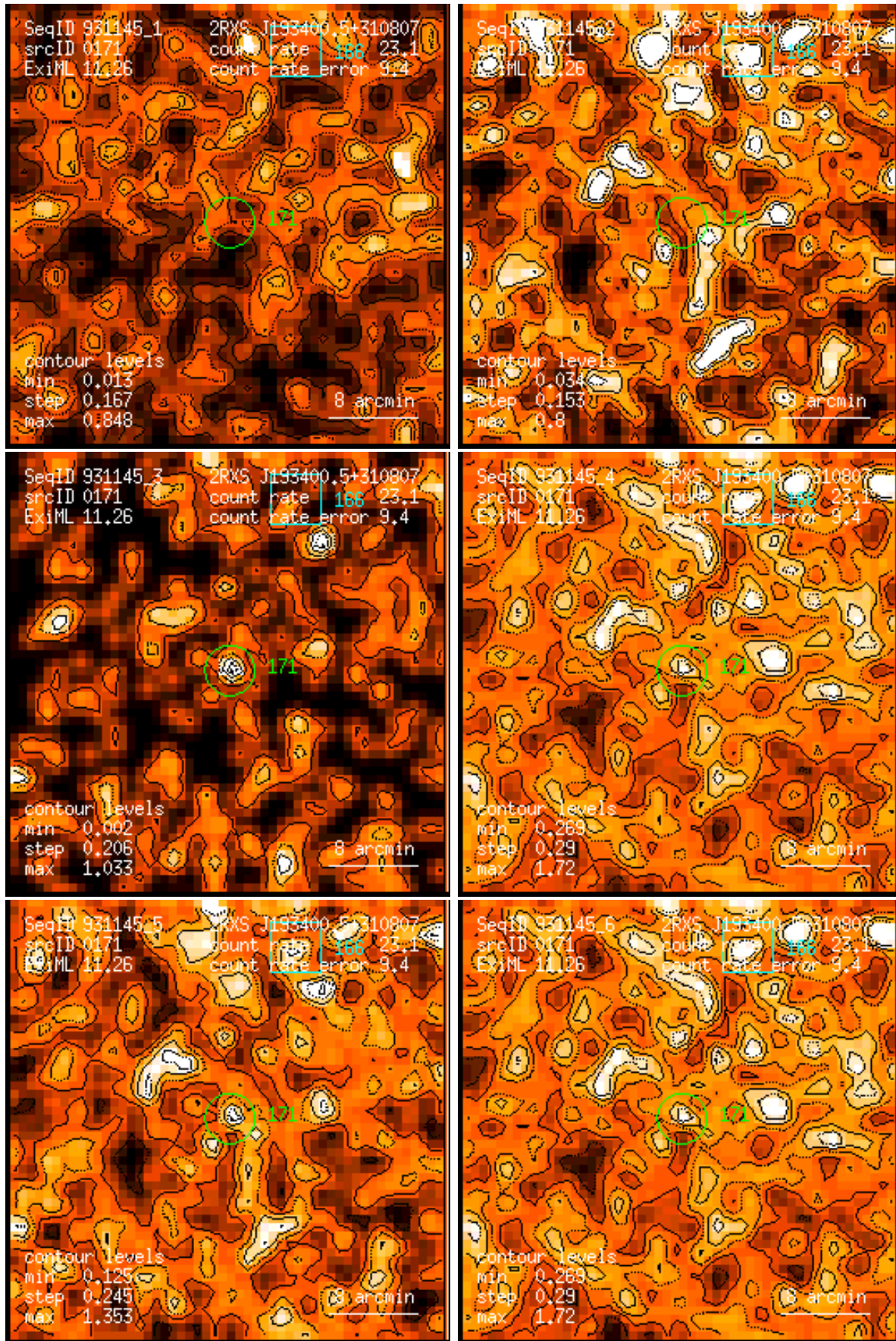
Figure 171: RASS 931145: detection 0171: band rate images, Gaussian filter: (1) PSPC channels 11 – 41, (2) 52 – 90, (3) 91 – 201, (4) 11 – 235, (5) 52 – 201, (6) 11 – 201. Broad band rates in counts/ks. Band rate contour levels in counts/ks/arcmin 2 .
