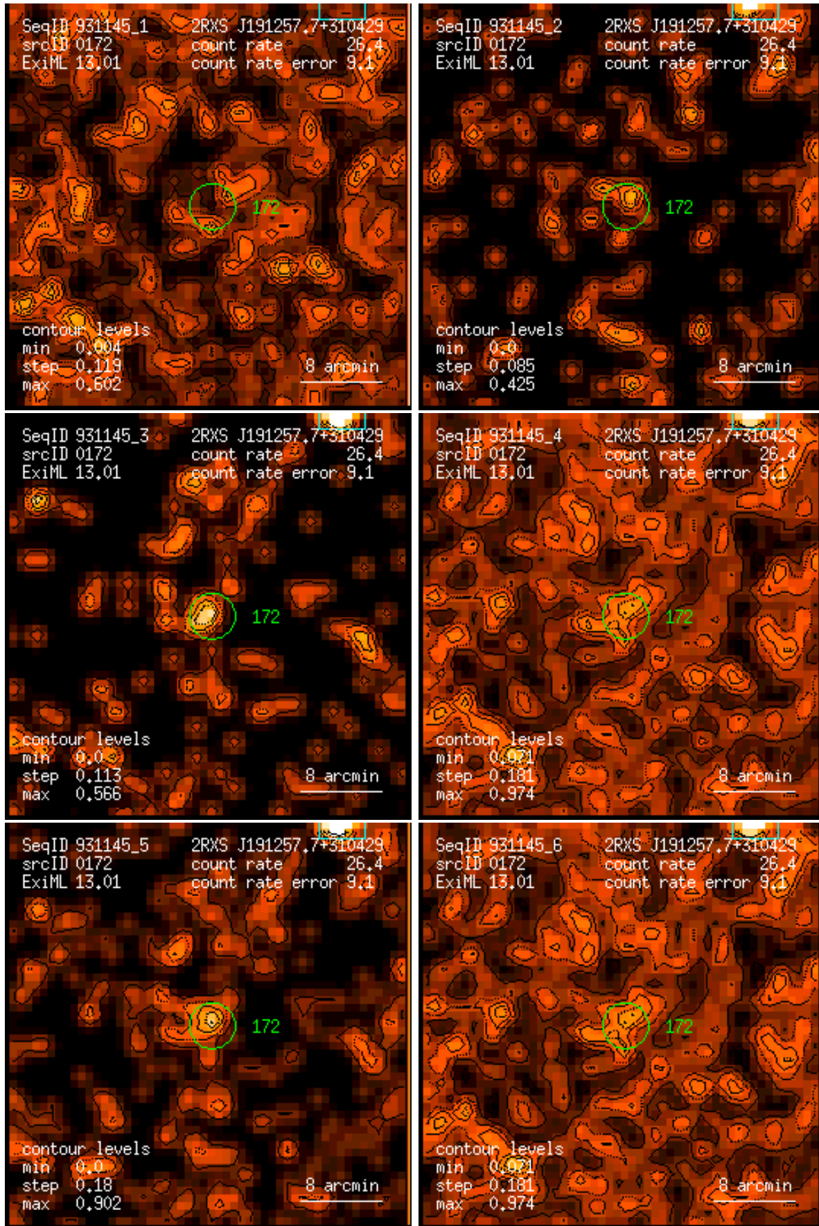
Figure 172: RASS 931145: detection 0172: band rate images, Gaussian filter: (1) PSPC channels 11 – 41, (2) 52 – 90, (3) 91 – 201, (4) 11 – 235, (5) 52 – 201, (6) 11 – 201. Broad band rates in counts/ks. Band rate contour levels in counts/ks/arcmin 2 .
