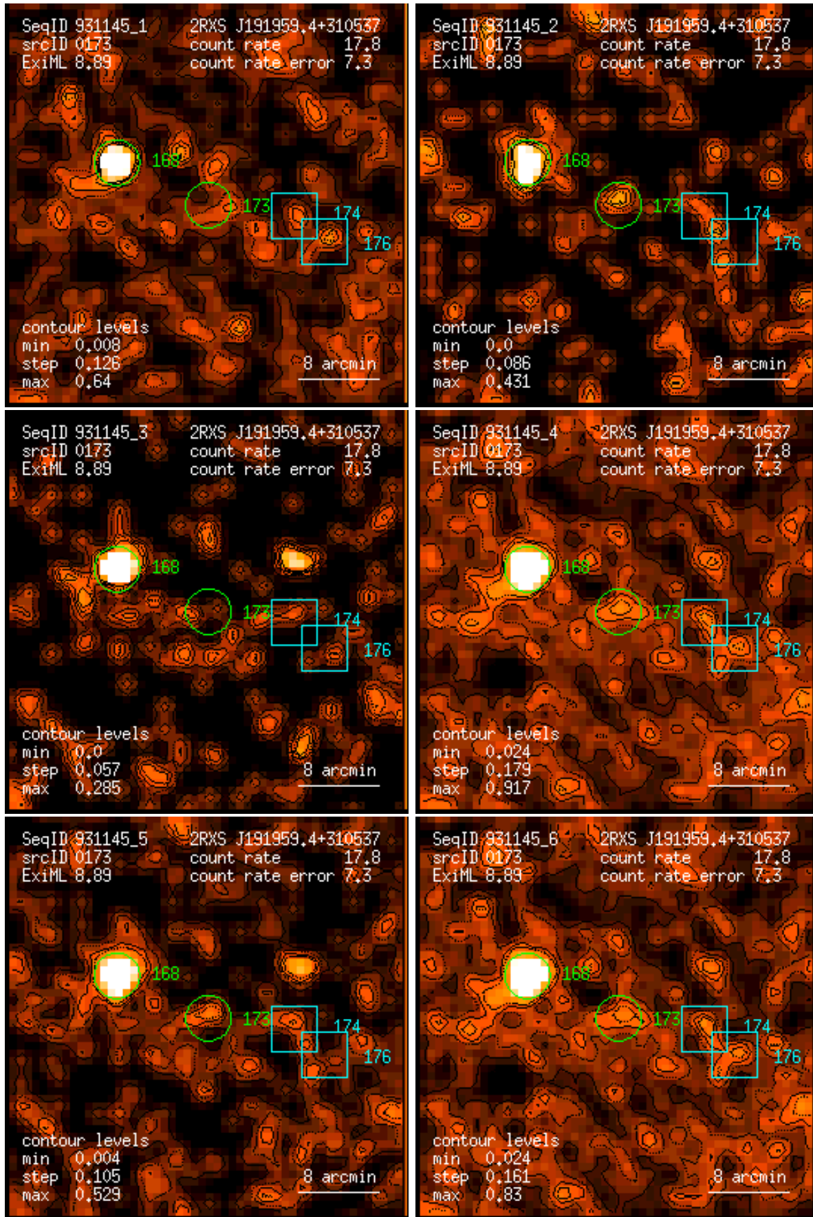
Figure 173: RASS 931145: detection 0173: band rate images, Gaussian filter: (1) PSPC channels 11 – 41, (2) 52 – 90, (3) 91 – 201, (4) 11 – 235, (5) 52 – 201, (6) 11 – 201. Broad band rates in counts/ks. Band rate contour levels in counts/ks/arcmin 2 .
