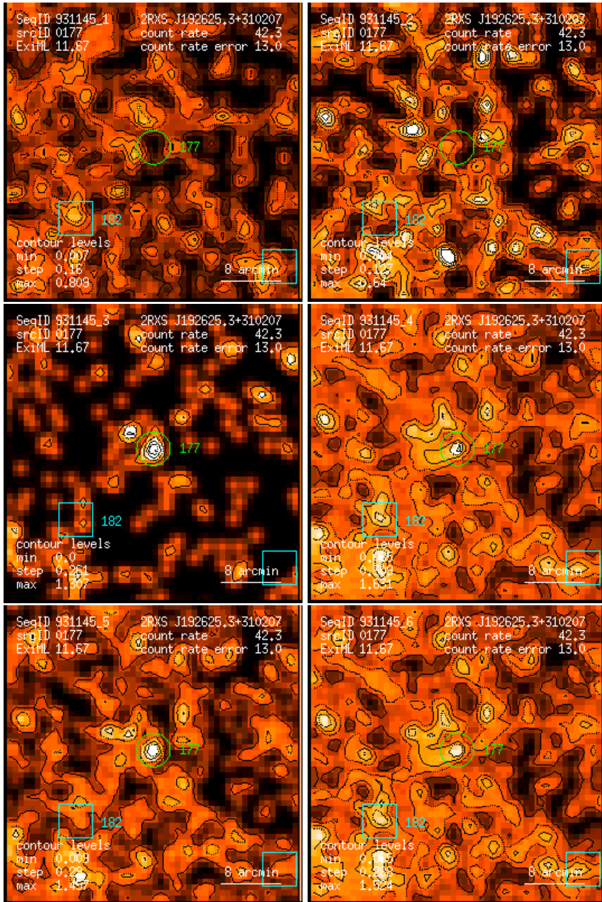
Figure 177: RASS 931145: detection 0177: band rate images, Gaussian filter: (1) PSPC channels 11 – 41, (2) 52 – 90, (3) 91 – 201, (4) 11 – 235, (5) 52 – 201, (6) 11 – 201. Broad band rates in counts/ks. Band rate contour levels in counts/ks/arcmin 2 .
