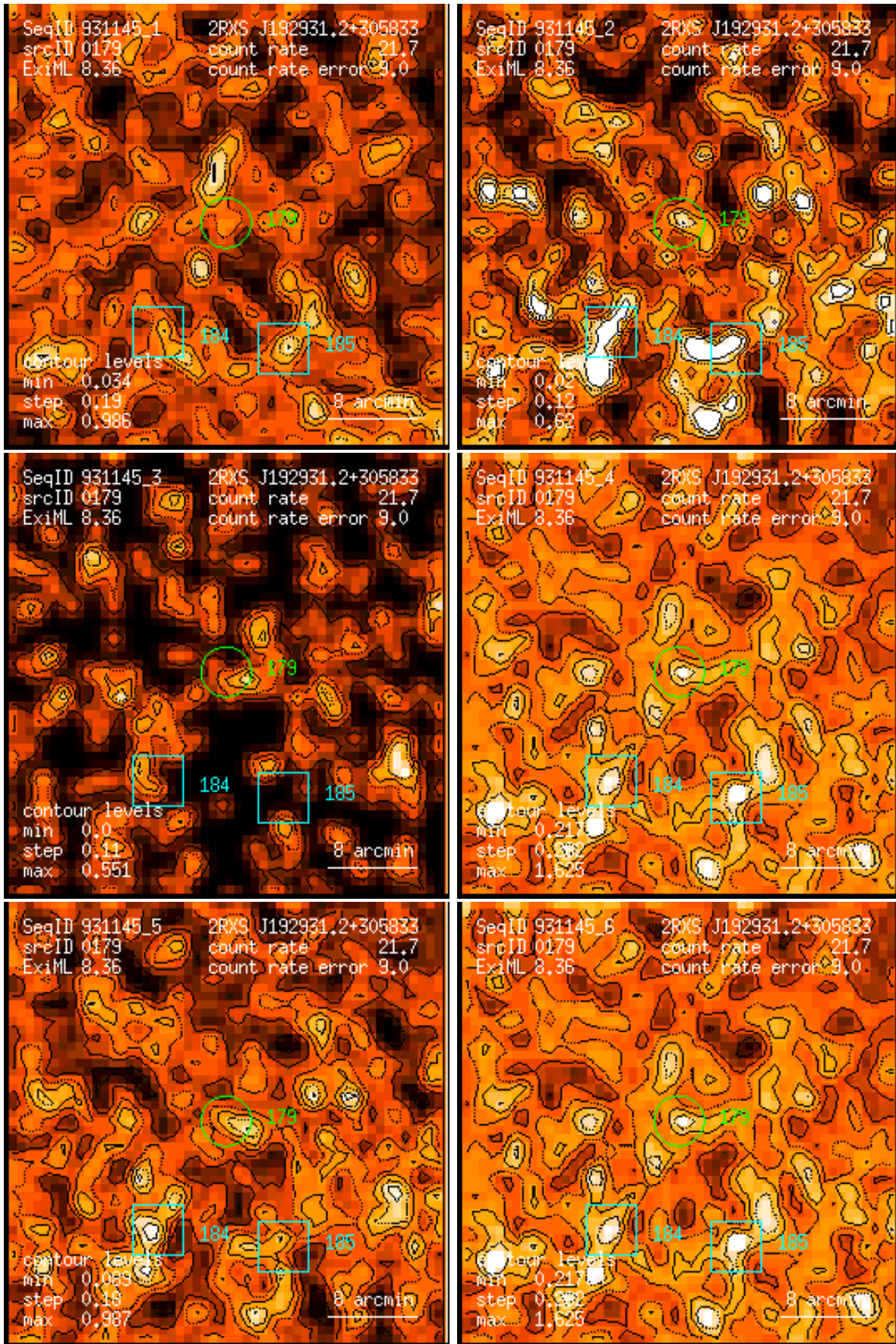
Figure 179: RASS 931145: detection 0179: band rate images, Gaussian filter: (1) PSPC channels 11 – 41, (2) 52 – 90, (3) 91 – 201, (4) 11 – 235, (5) 52 – 201, (6) 11 – 201. Broad band rates in counts/ks. Band rate contour levels in counts/ks/arcmin 2 .
