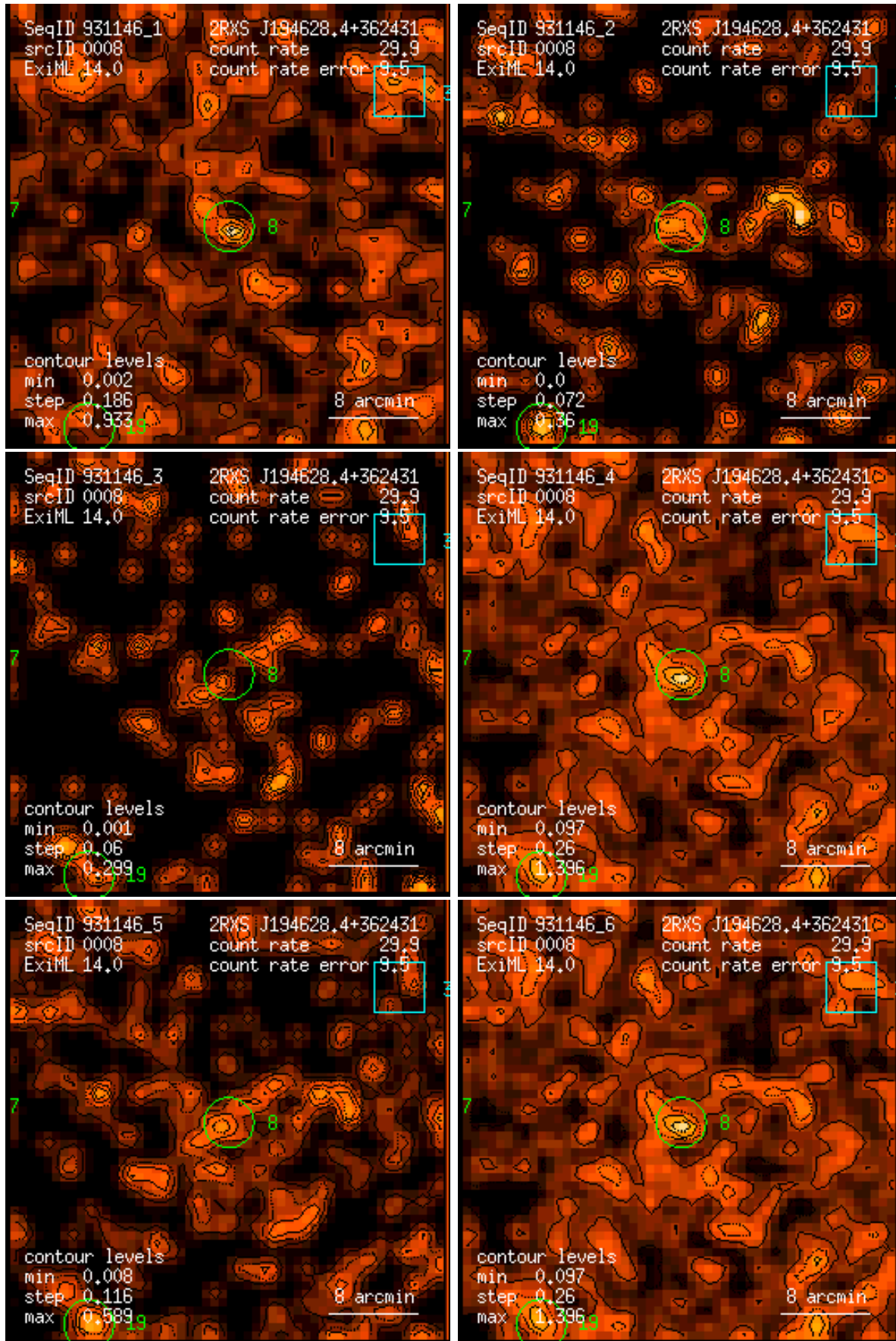
Figure 8: RASS 931146: detection 0008: band rate images, Gaussian filter: (1) PSPC channels 11 – 41, (2) 52 – 90, (3) 91 – 201, (4) 11 – 235, (5) 52 – 201, (6) 11 – 201. Broad band rates in counts/ks. Band rate contour levels in counts/ks/arcmin 2 .
