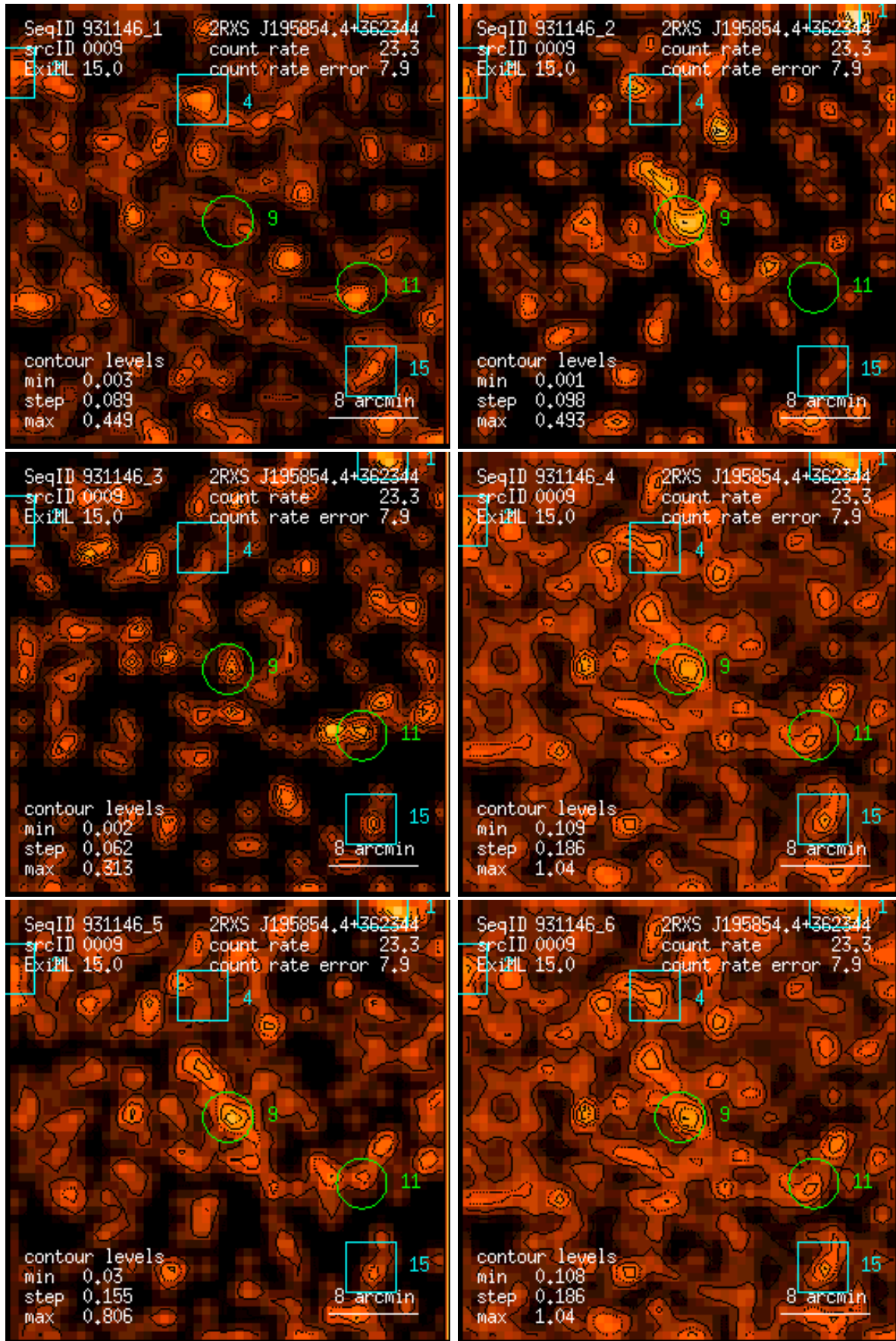
Figure 9: RASS 931146: detection 0009: band rate images, Gaussian filter: (1) PSPC channels 11 – 41, (2) 52 – 90, (3) 91 – 201, (4) 11 – 235, (5) 52 – 201, (6) 11 – 201. Broad band rates in counts/ks. Band rate contour levels in counts/ks/arcmin 2 .
