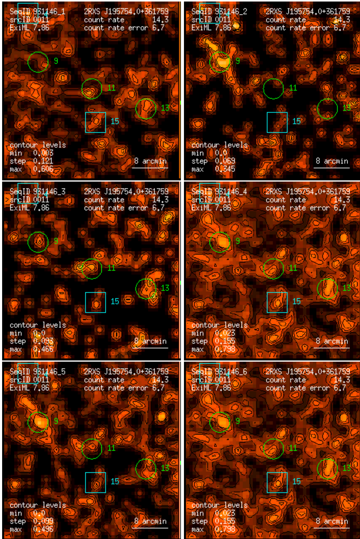
Figure 11: RASS 931146: detection 0011: band rate images, Gaussian filter: (1) PSPC channels 11 – 41, (2) 52 – 90, (3) 91 – 201, (4) 11 – 235, (5) 52 – 201, (6) 11 – 201. Broad band rates in counts/ks. Band rate contour levels in counts/ks/arcmin 2 .
