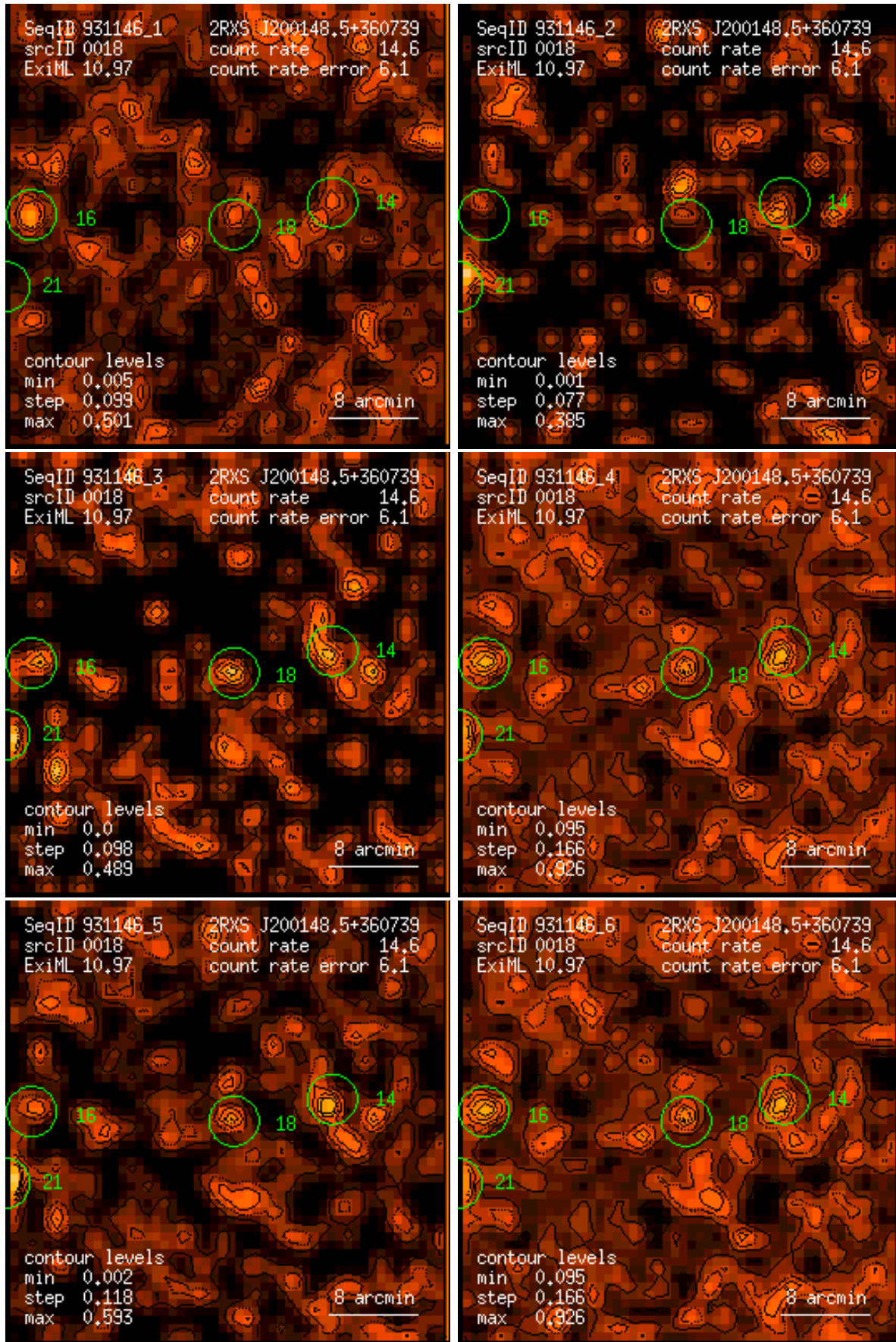
Figure 18: RASS 931146: detection 0018: band rate images, Gaussian filter: (1) PSPC channels 11 – 41, (2) 52 – 90, (3) 91 – 201, (4) 11 – 235, (5) 52 – 201, (6) 11 – 201. Broad band rates in counts/ks. Band rate contour levels in counts/ks/arcmin 2 .
