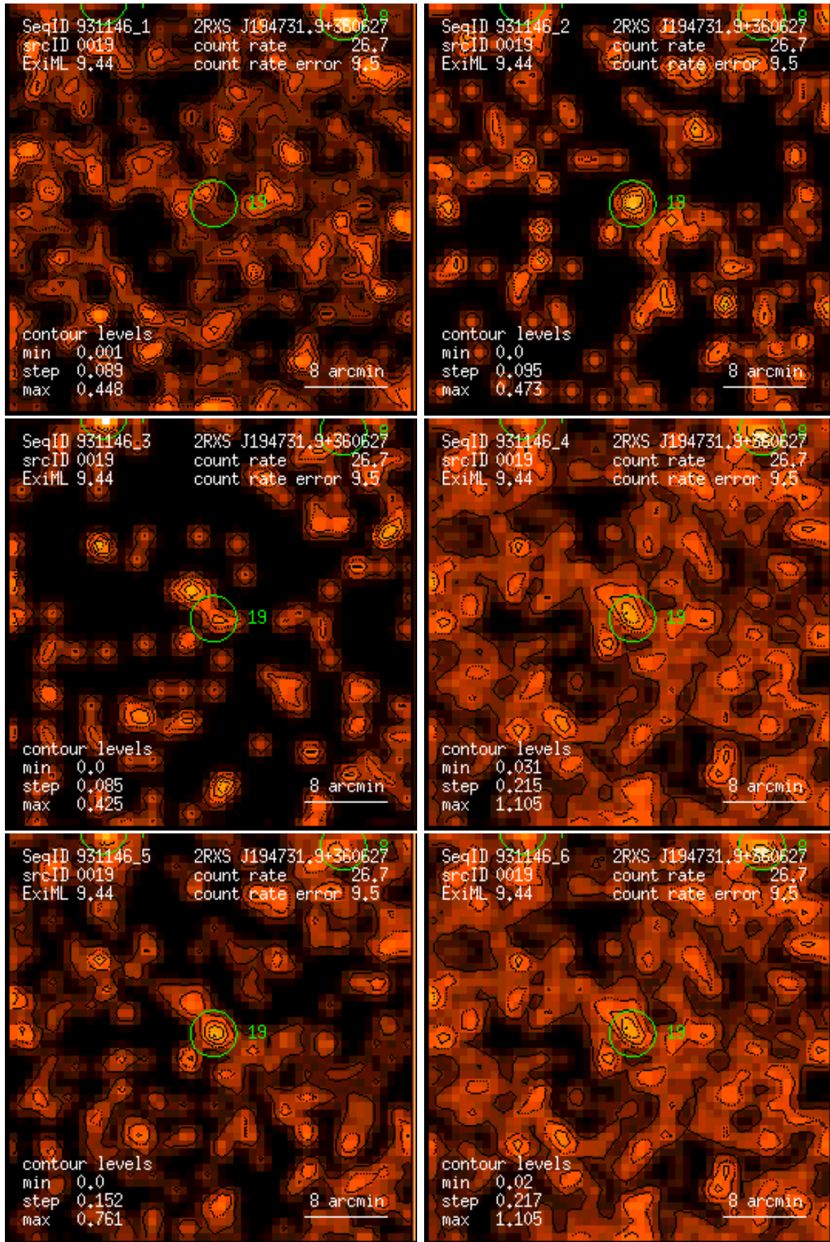
Figure 19: RASS 931146: detection 0019: band rate images, Gaussian filter: (1) PSPC channels 11 – 41, (2) 52 – 90, (3) 91 – 201, (4) 11 – 235, (5) 52 – 201, (6) 11 – 201. Broad band rates in counts/ks. Band rate contour levels in counts/ks/arcmin 2 .
