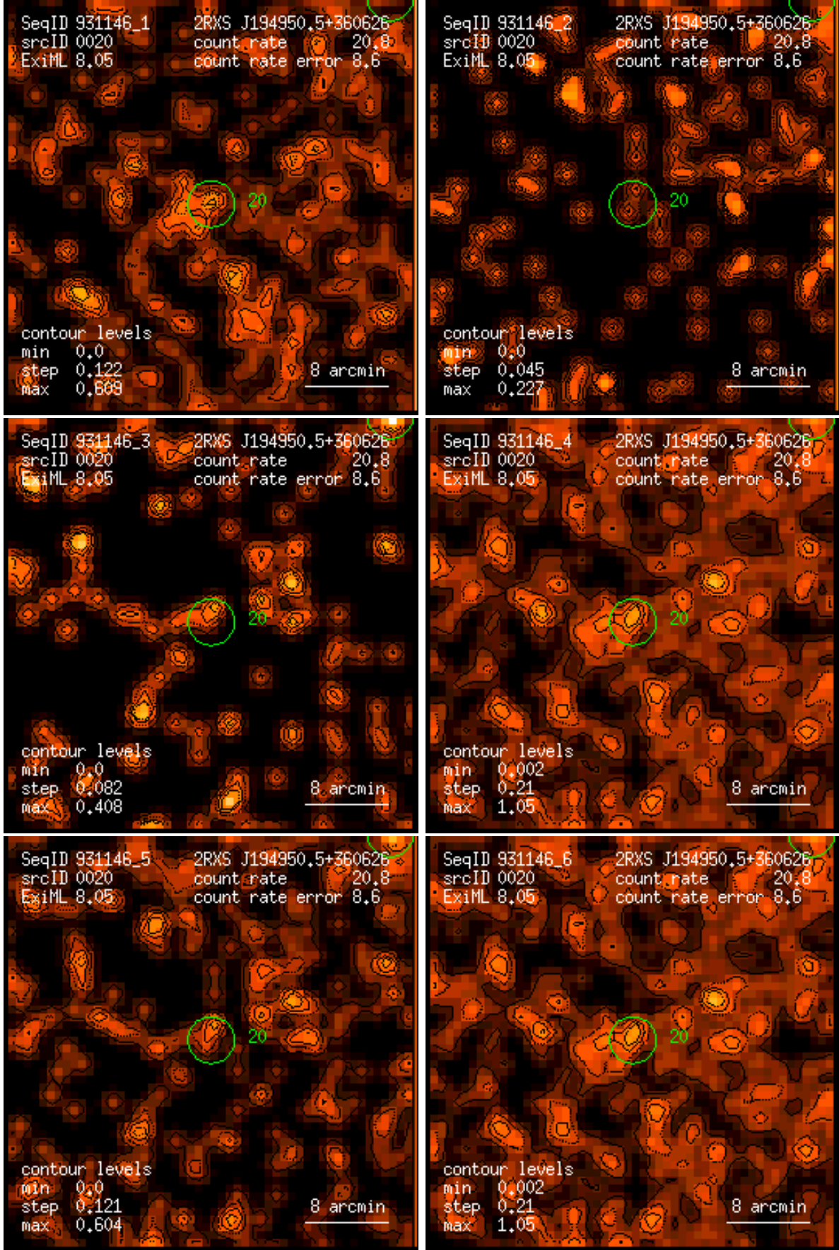
Figure 20: RASS 931146: detection 0020: band rate images, Gaussian filter: (1) PSPC channels 11 – 41, (2) 52 – 90, (3) 91 – 201, (4) 11 – 235, (5) 52 – 201, (6) 11 – 201. Broad band rates in counts/ks. Band rate contour levels in counts/ks/arcmin 2 .
