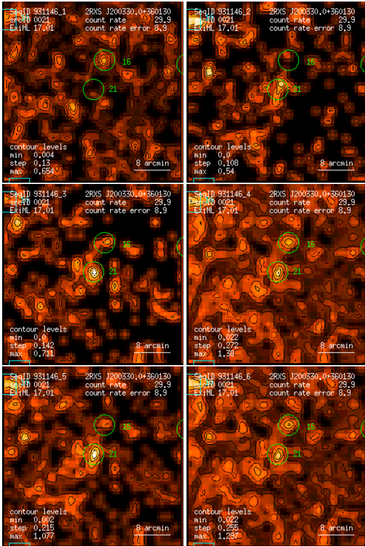
Figure 21: RASS 931146: detection 0021: band rate images, Gaussian filter: (1) PSPC channels 11 – 41, (2) 52 – 90, (3) 91 – 201, (4) 11 – 235, (5) 52 – 201, (6) 11 – 201. Broad band rates in counts/ks. Band rate contour levels in counts/ks/arcmin 2 .
