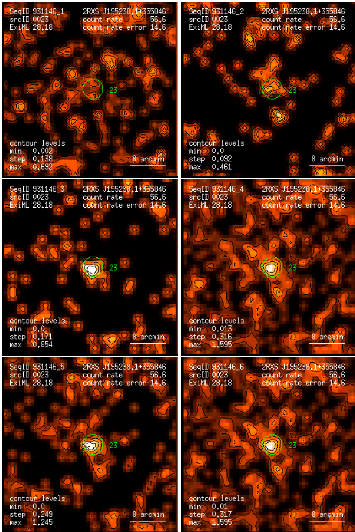
Figure 23: RASS 931146: detection 0023: band rate images, Gaussian filter: (1) PSPC channels 11 – 41, (2) 52 – 90, (3) 91 – 201, (4) 11 – 235, (5) 52 – 201, (6) 11 – 201. Broad band rates in counts/ks. Band rate contour levels in counts/ks/arcmin 2 .
