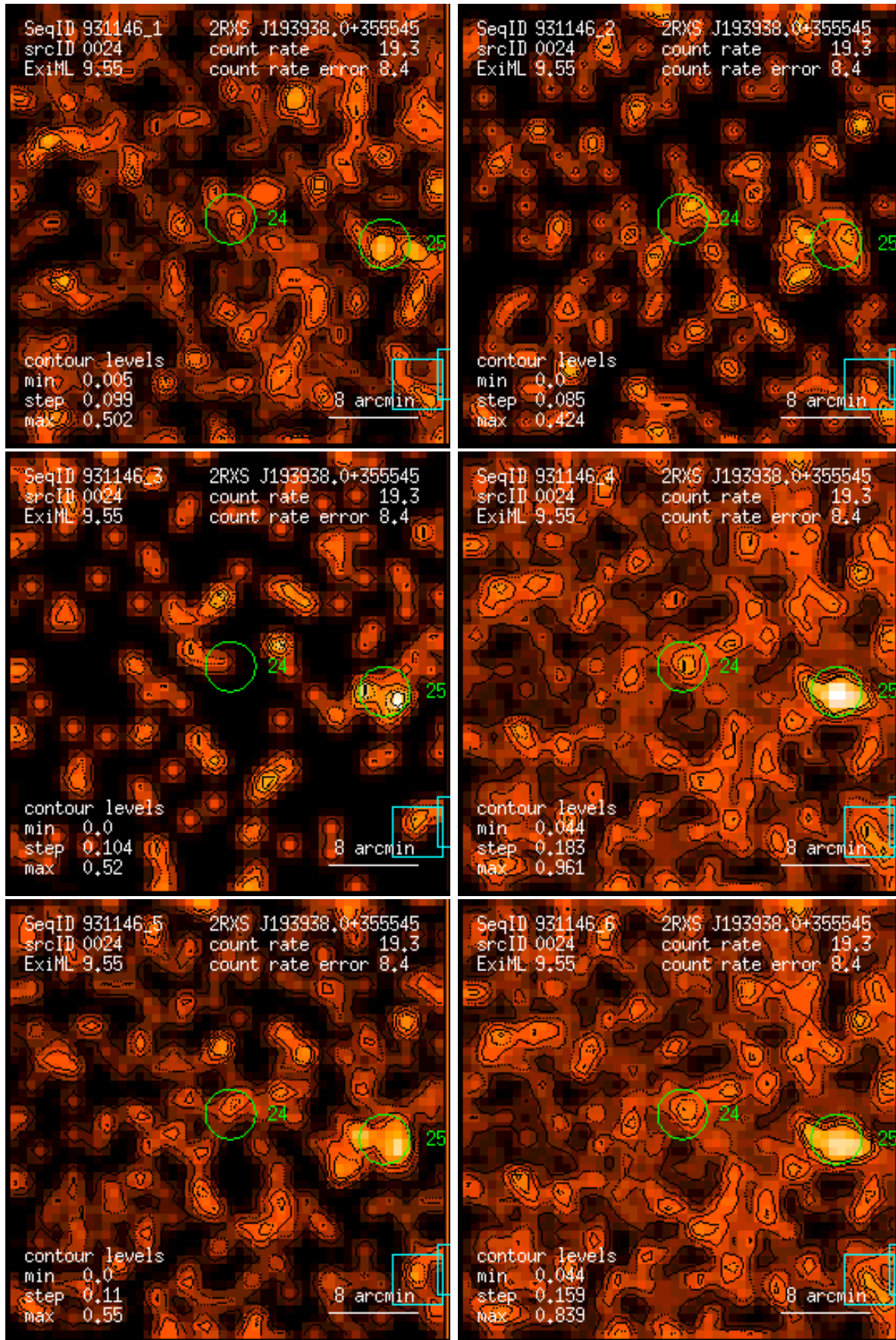
Figure 24: RASS 931146: detection 0024: band rate images, Gaussian filter: (1) PSPC channels 11 – 41, (2) 52 – 90, (3) 91 – 201, (4) 11 – 235, (5) 52 – 201, (6) 11 – 201. Broad band rates in counts/ks. Band rate contour levels in counts/ks/arcmin 2 .
