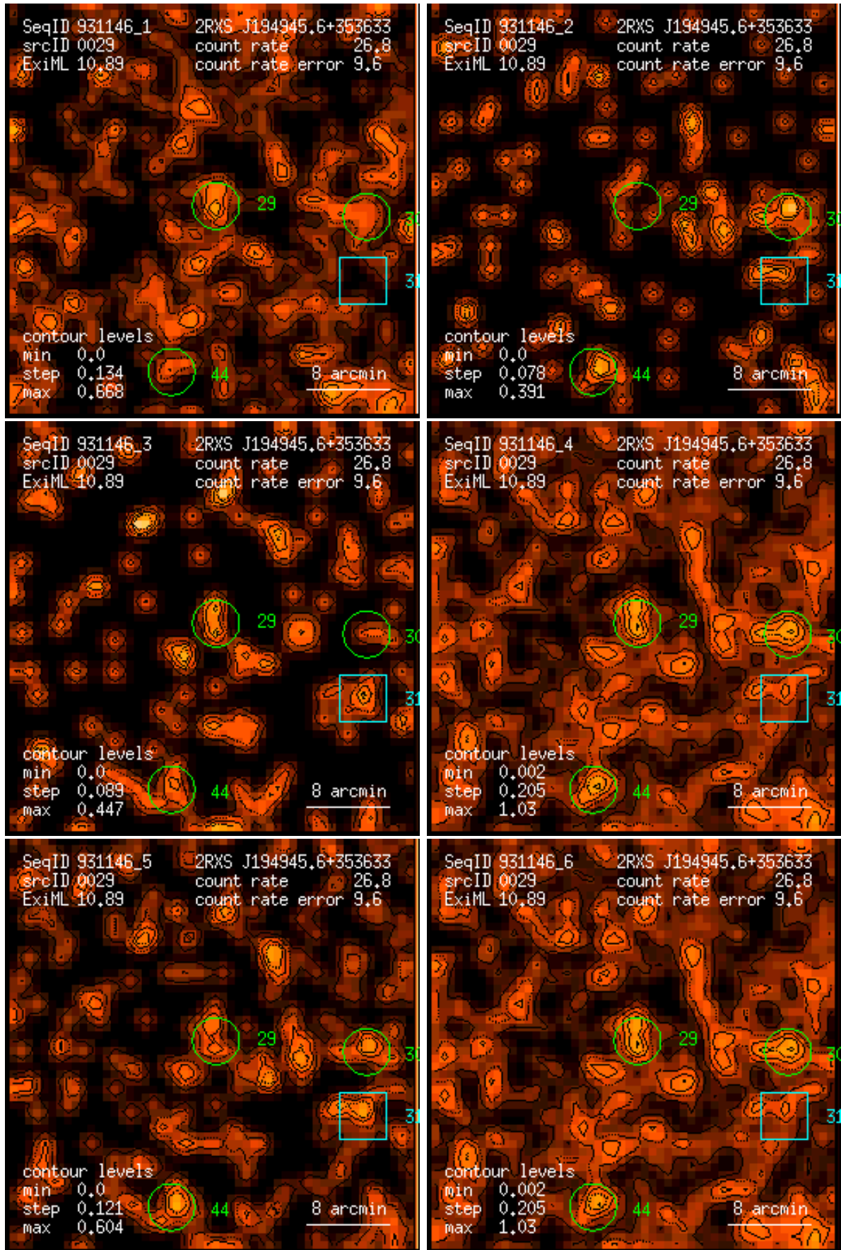
Figure 29: RASS 931146: detection 0029: band rate images, Gaussian filter: (1) PSPC channels 11 – 41, (2) 52 – 90, (3) 91 – 201, (4) 11 – 235, (5) 52 – 201, (6) 11 – 201. Broad band rates in counts/ks. Band rate contour levels in counts/ks/arcmin 2 .
