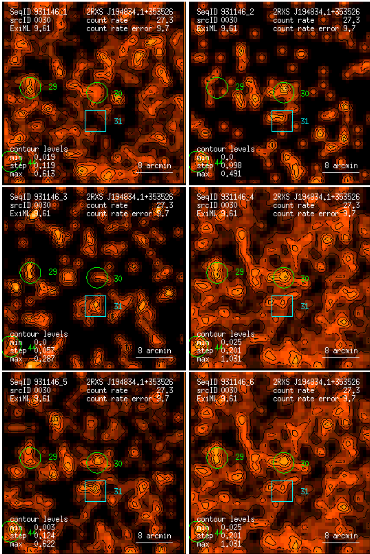
Figure 30: RASS 931146: detection 0030: band rate images, Gaussian filter: (1) PSPC channels 11 – 41, (2) 52 – 90, (3) 91 – 201, (4) 11 – 235, (5) 52 – 201, (6) 11 – 201. Broad band rates in counts/ks. Band rate contour levels in counts/ks/arcmin 2 .
