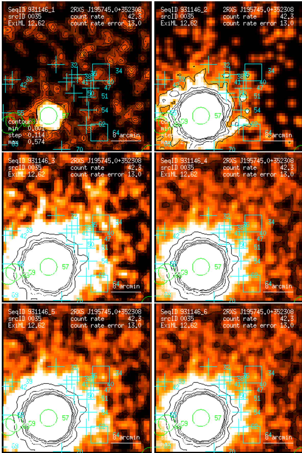
Figure 35: RASS 931146: detection 0035: band rate images, Gaussian filter: (1) PSPC channels 11 – 41, (2) 52 – 90, (3) 91 – 201, (4) 11 – 235, (5) 52 – 201, (6) 11 – 201. Broad band rates in counts/ks. Band rate contour levels in counts/ks/arcmin 2 .
