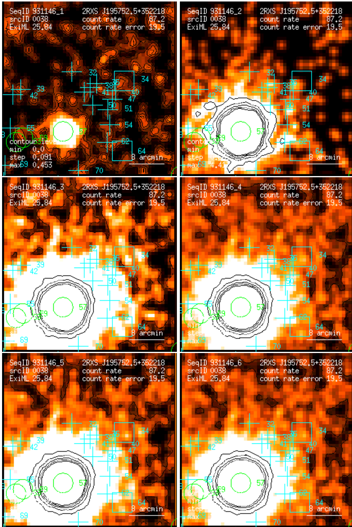
Figure 38: RASS 931146: detection 0038: band rate images, Gaussian filter: (1) PSPC channels 11 – 41, (2) 52 – 90, (3) 91 – 201, (4) 11 – 235, (5) 52 – 201, (6) 11 – 201. Broad band rates in counts/ks. Band rate contour levels in counts/ks/arcmin 2 .
