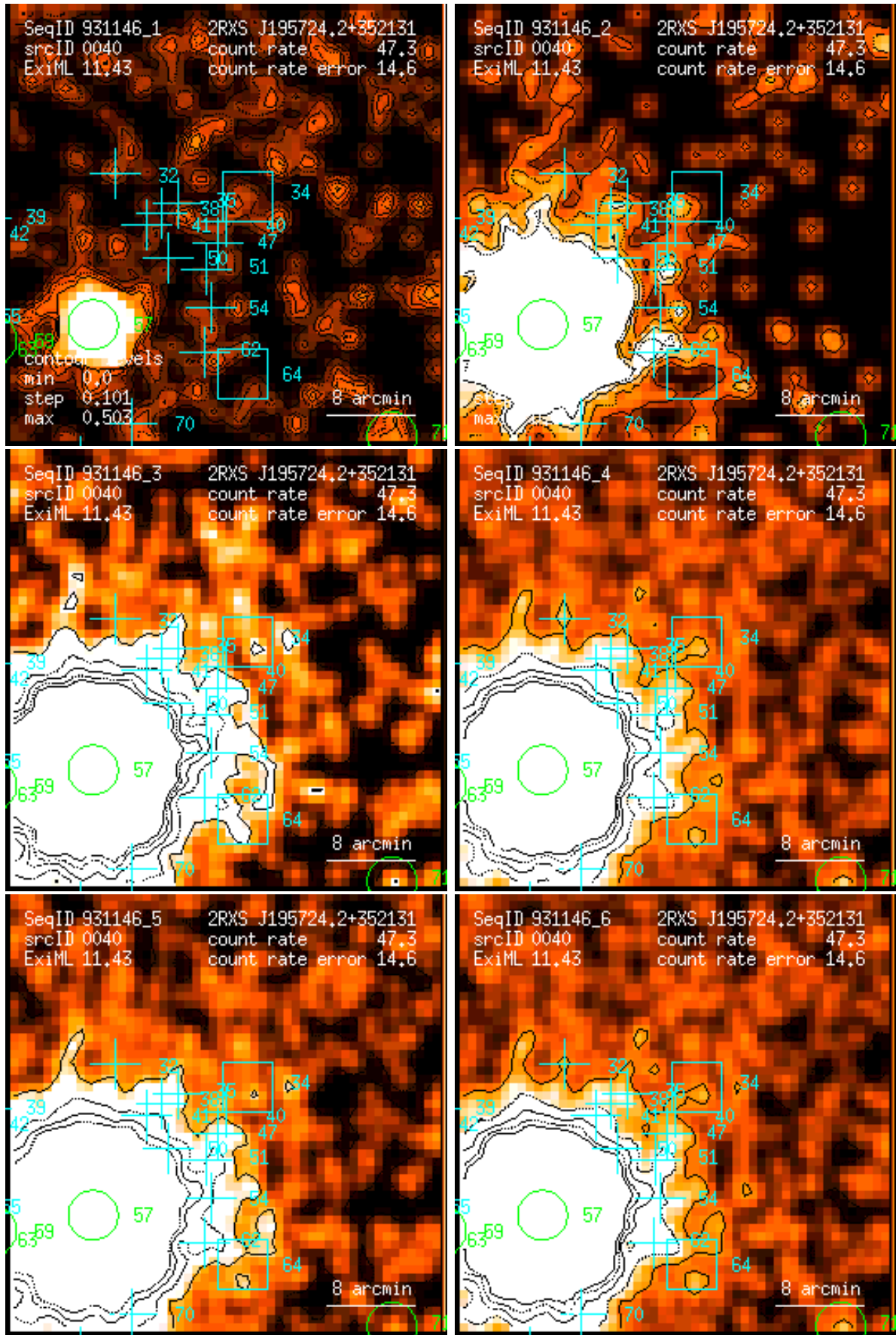
Figure 40: RASS 931146: detection 0040: band rate images, Gaussian filter: (1) PSPC channels 11 – 41, (2) 52 – 90, (3) 91 – 201, (4) 11 – 235, (5) 52 – 201, (6) 11 – 201. Broad band rates in counts/ks. Band rate contour levels in counts/ks/arcmin 2 .
