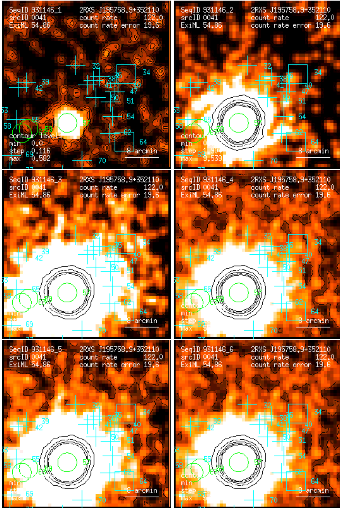
Figure 41: RASS 931146: detection 0041: band rate images, Gaussian filter: (1) PSPC channels 11 – 41, (2) 52 – 90, (3) 91 – 201, (4) 11 – 235, (5) 52 – 201, (6) 11 – 201. Broad band rates in counts/ks. Band rate contour levels in counts/ks/arcmin 2 .
