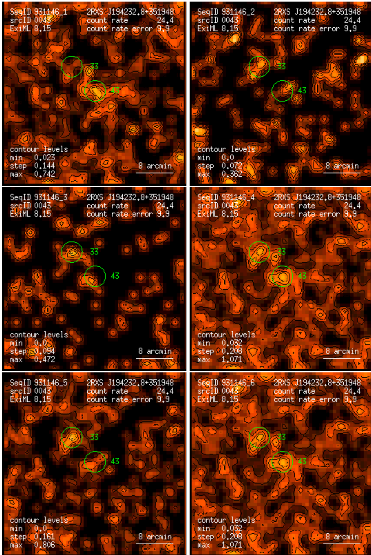
Figure 43: RASS 931146: detection 0043: band rate images, Gaussian filter: (1) PSPC channels 11 – 41, (2) 52 – 90, (3) 91 – 201, (4) 11 – 235, (5) 52 – 201, (6) 11 – 201. Broad band rates in counts/ks. Band rate contour levels in counts/ks/arcmin 2 .
