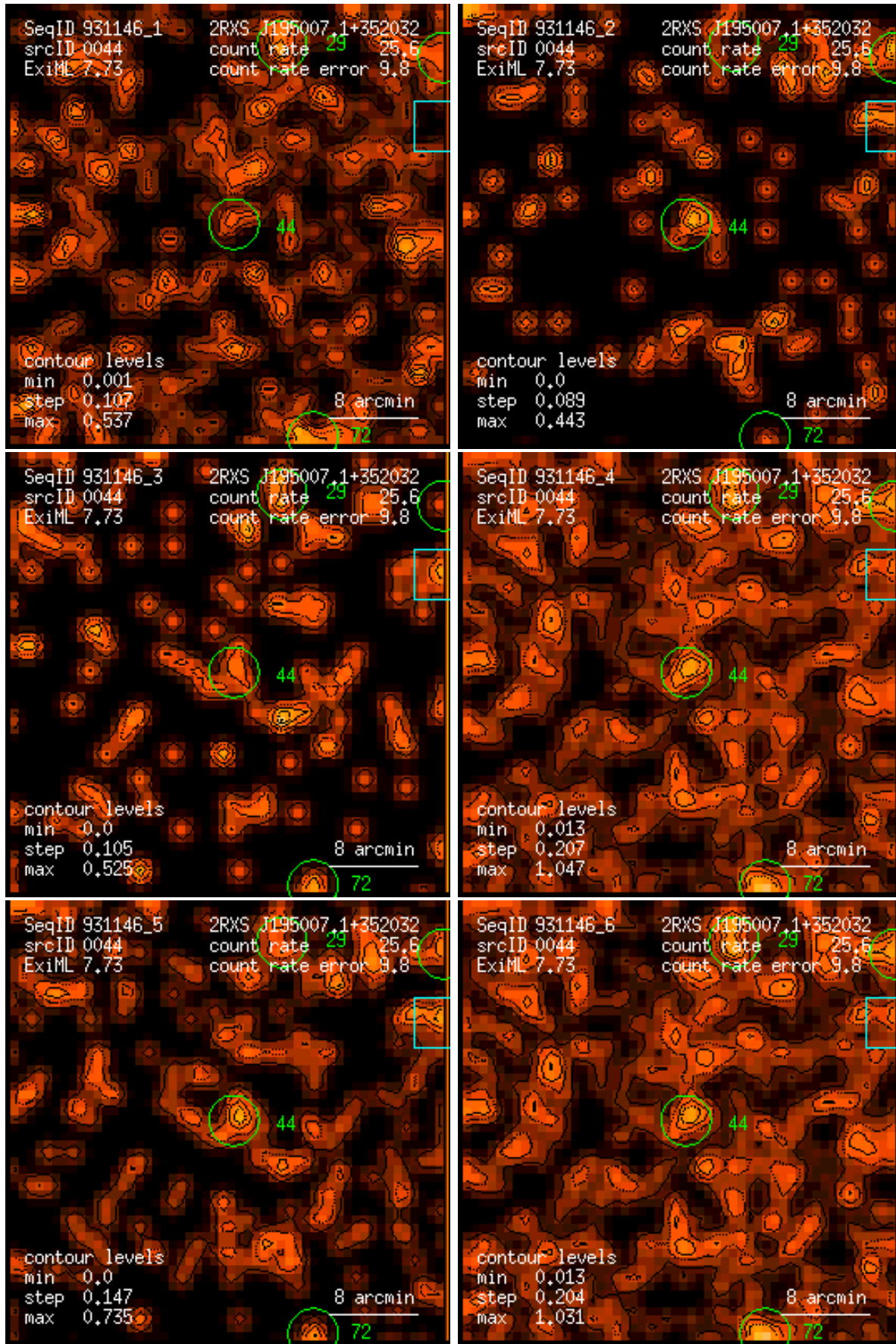
Figure 44: RASS 931146: detection 0044: band rate images, Gaussian filter: (1) PSPC channels 11 – 41, (2) 52 – 90, (3) 91 – 201, (4) 11 – 235, (5) 52 – 201, (6) 11 – 201. Broad band rates in counts/ks. Band rate contour levels in counts/ks/arcmin 2 .
