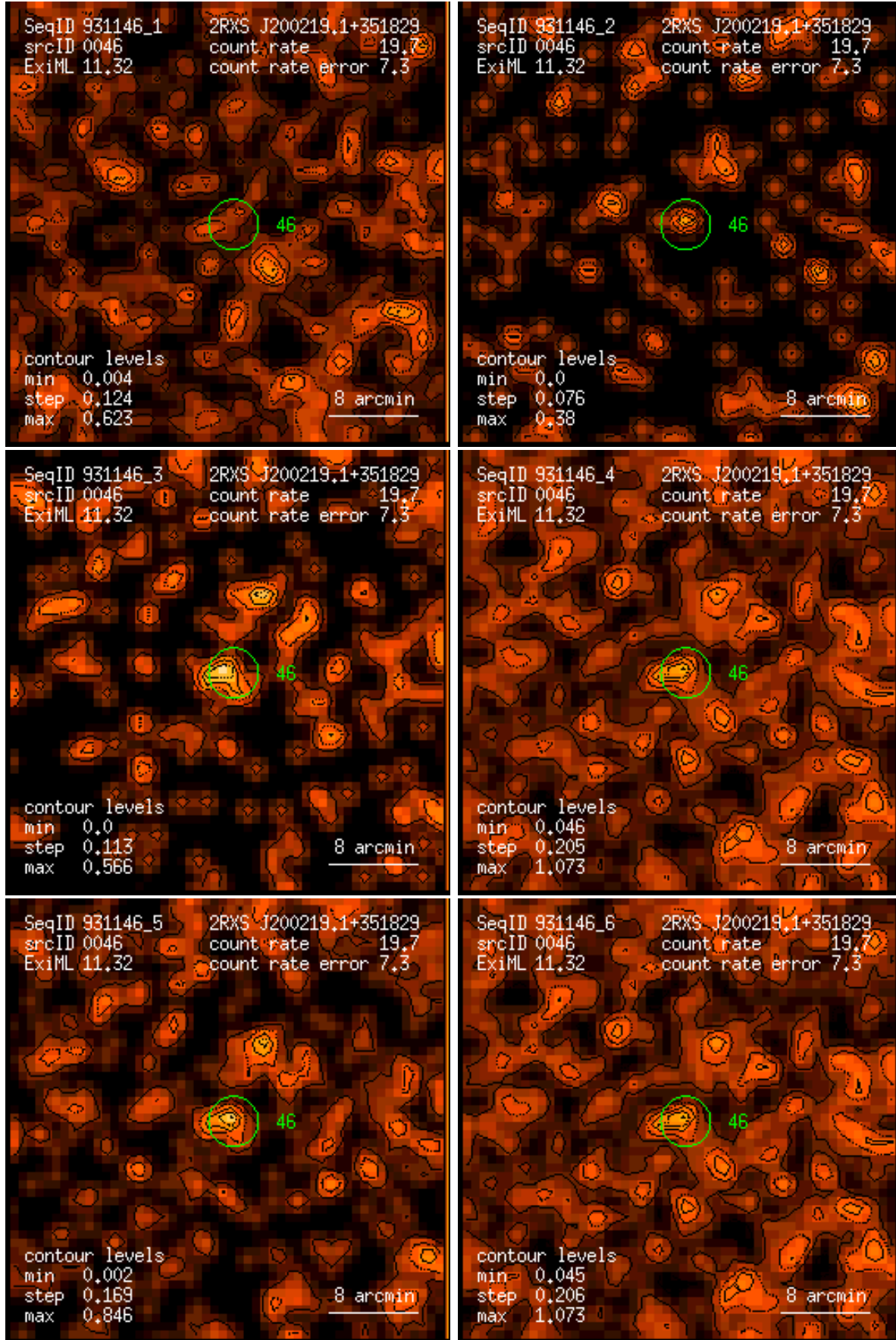
Figure 46: RASS 931146: detection 0046: band rate images, Gaussian filter: (1) PSPC channels 11 – 41, (2) 52 – 90, (3) 91 – 201, (4) 11 – 235, (5) 52 – 201, (6) 11 – 201. Broad band rates in counts/ks. Band rate contour levels in counts/ks/arcmin 2 .
