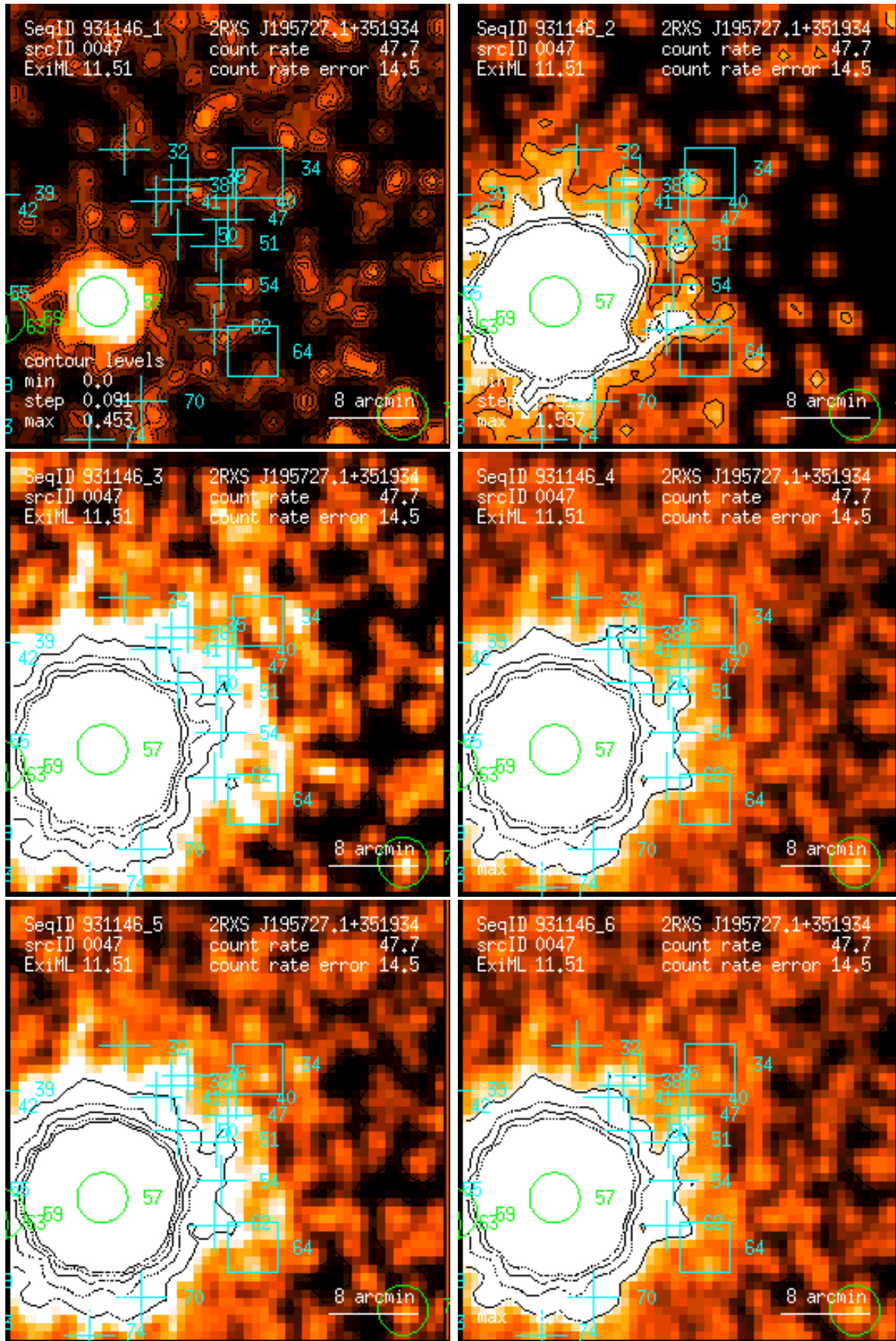
Figure 47: RASS 931146: detection 0047: band rate images, Gaussian filter: (1) PSPC channels 11 – 41, (2) 52 – 90, (3) 91 – 201, (4) 11 – 235, (5) 52 – 201, (6) 11 – 201. Broad band rates in counts/ks. Band rate contour levels in counts/ks/arcmin 2 .
