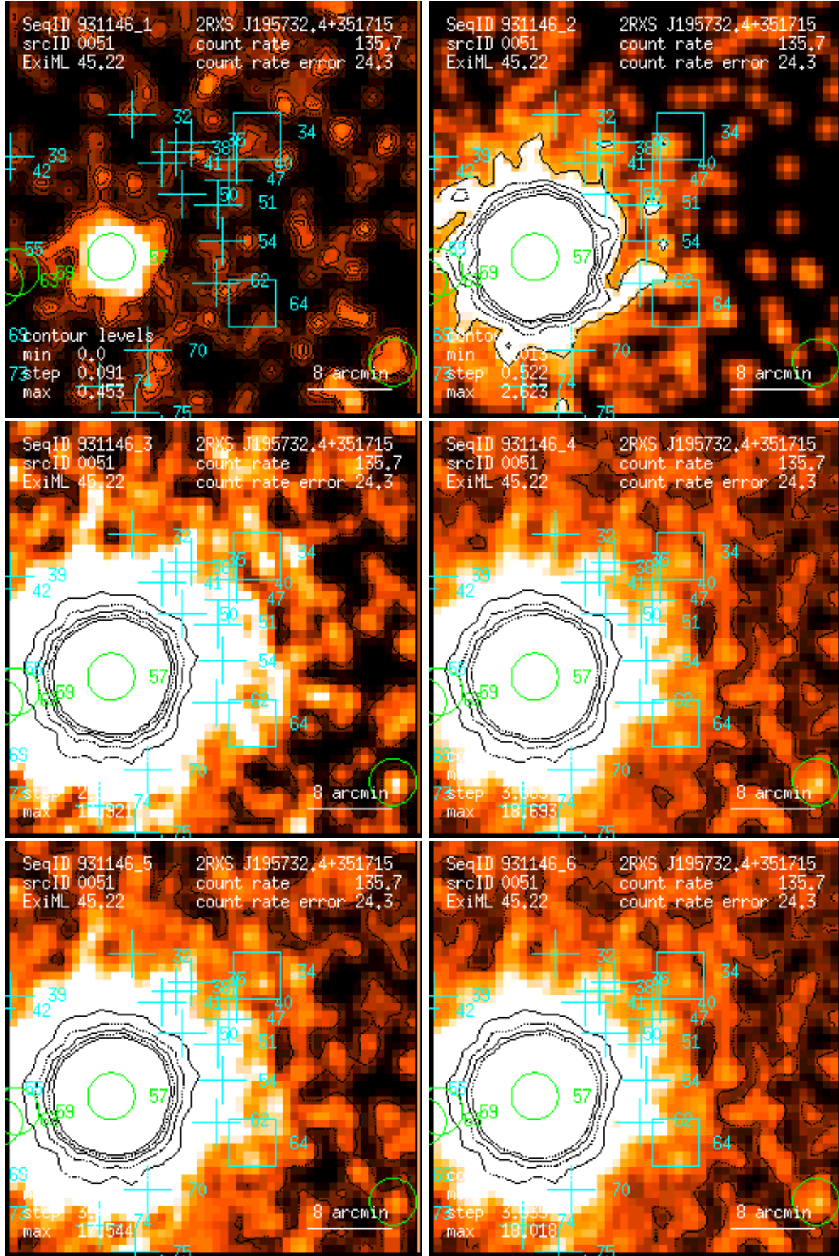
Figure 51: RASS 931146: detection 0051: band rate images, Gaussian filter: (1) PSPC channels 11 – 41, (2) 52 – 90, (3) 91 – 201, (4) 11 – 235, (5) 52 – 201, (6) 11 – 201. Broad band rates in counts/ks. Band rate contour levels in counts/ks/arcmin 2 .
