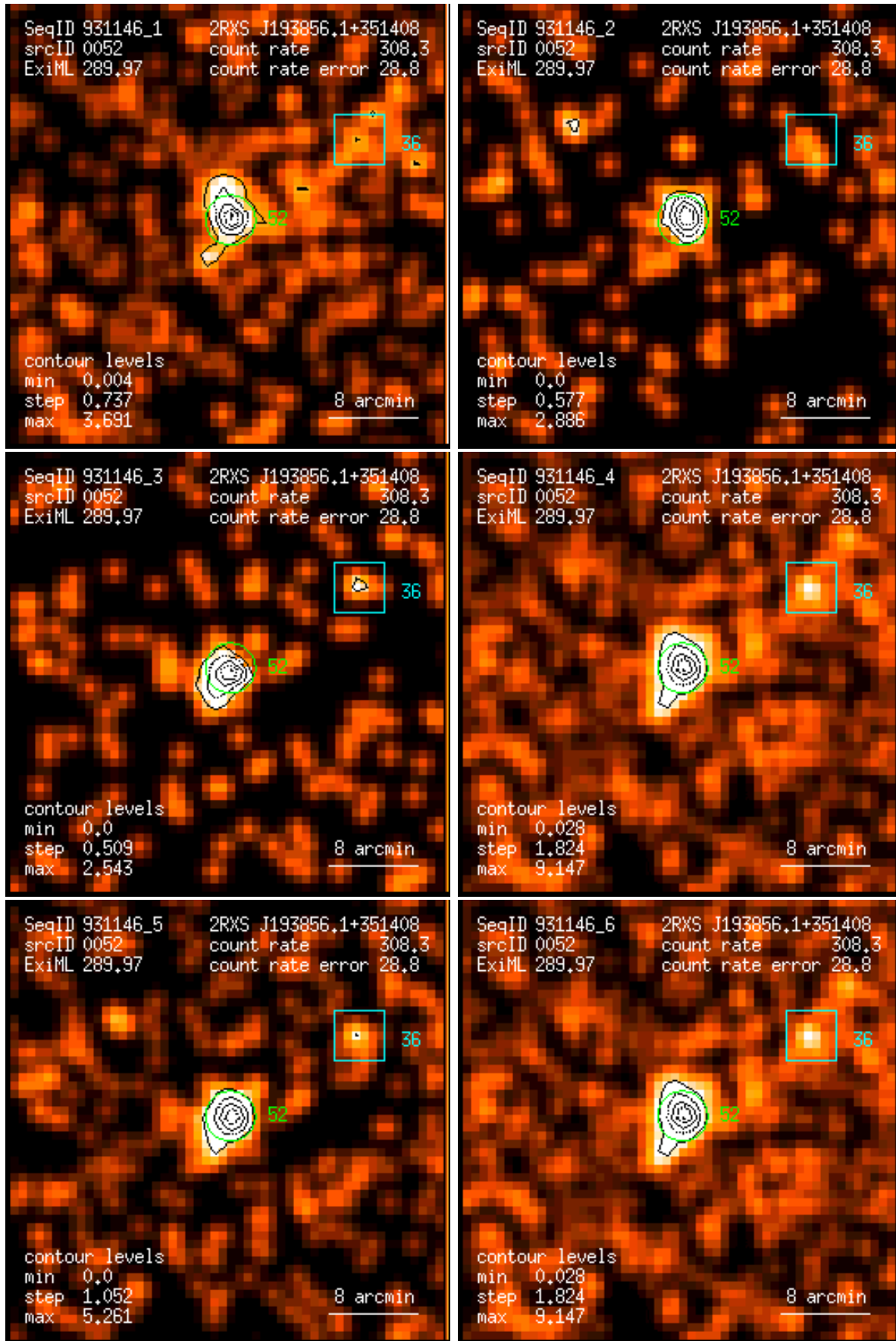
Figure 52: RASS 931146: detection 0052: band rate images, Gaussian filter: (1) PSPC channels 11 – 41, (2) 52 – 90, (3) 91 – 201, (4) 11 – 235, (5) 52 – 201, (6) 11 – 201. Broad band rates in counts/ks. Band rate contour levels in counts/ks/arcmin 2 .
