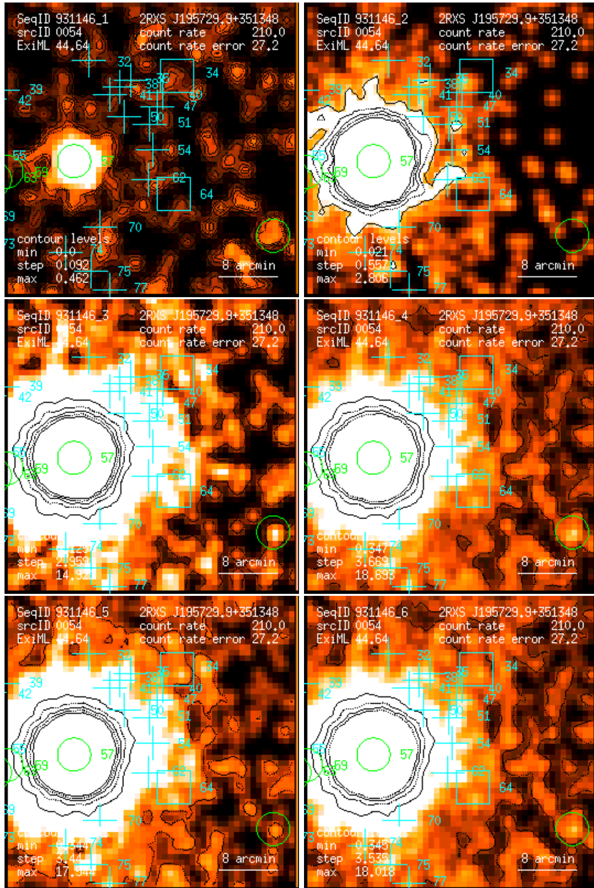
Figure 54: RASS 931146: detection 0054: band rate images, Gaussian filter: (1) PSPC channels 11 – 41, (2) 52 – 90, (3) 91 – 201, (4) 11 – 235, (5) 52 – 201, (6) 11 – 201. Broad band rates in counts/ks. Band rate contour levels in counts/ks/arcmin 2 .
