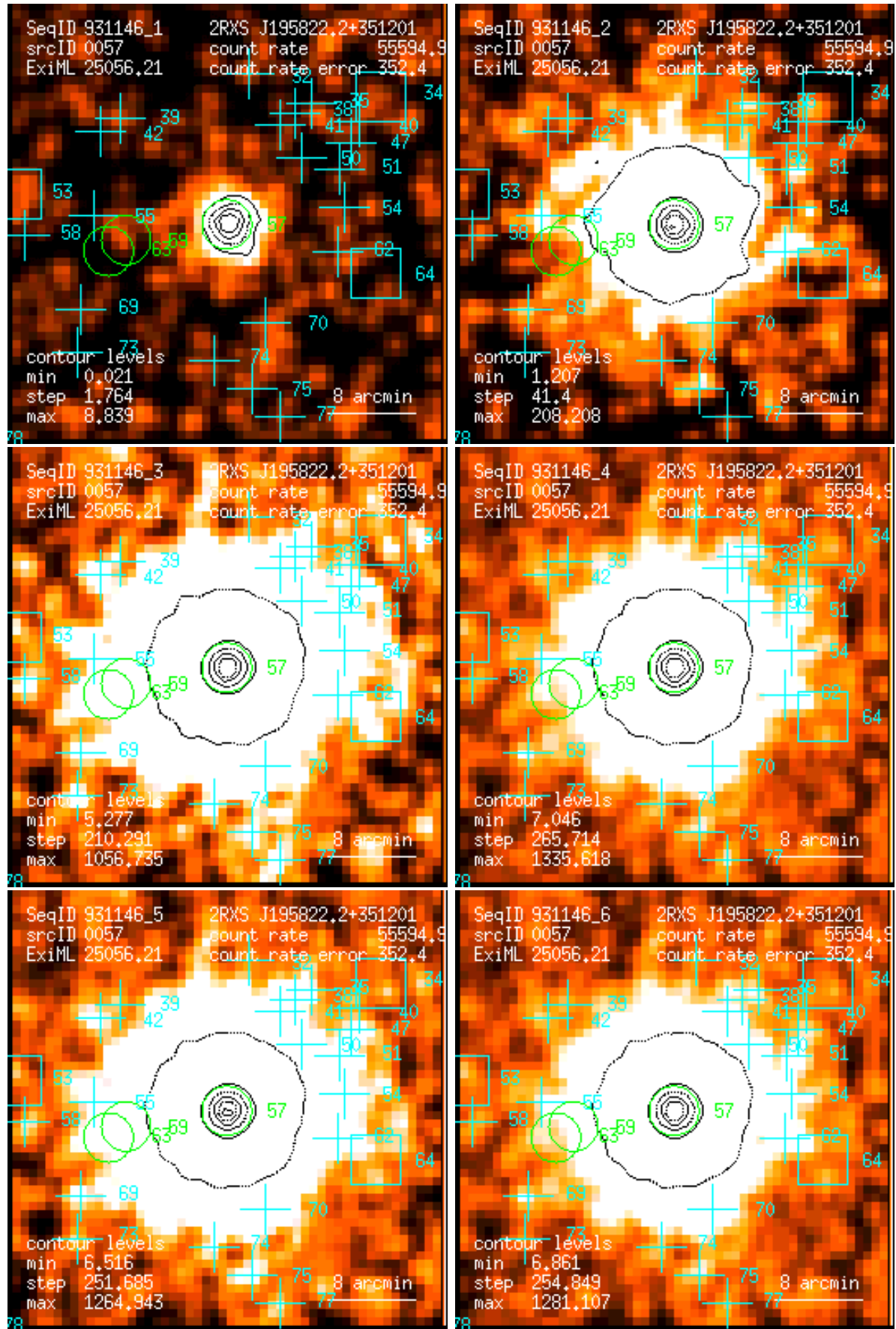
Figure 57: RASS 931146: detection 0057: band rate images, Gaussian filter: (1) PSPC channels 11 – 41, (2) 52 – 90, (3) 91 – 201, (4) 11 – 235, (5) 52 – 201, (6) 11 – 201. Broad band rates in counts/ks. Band rate contour levels in counts/ks/arcmin 2 .
