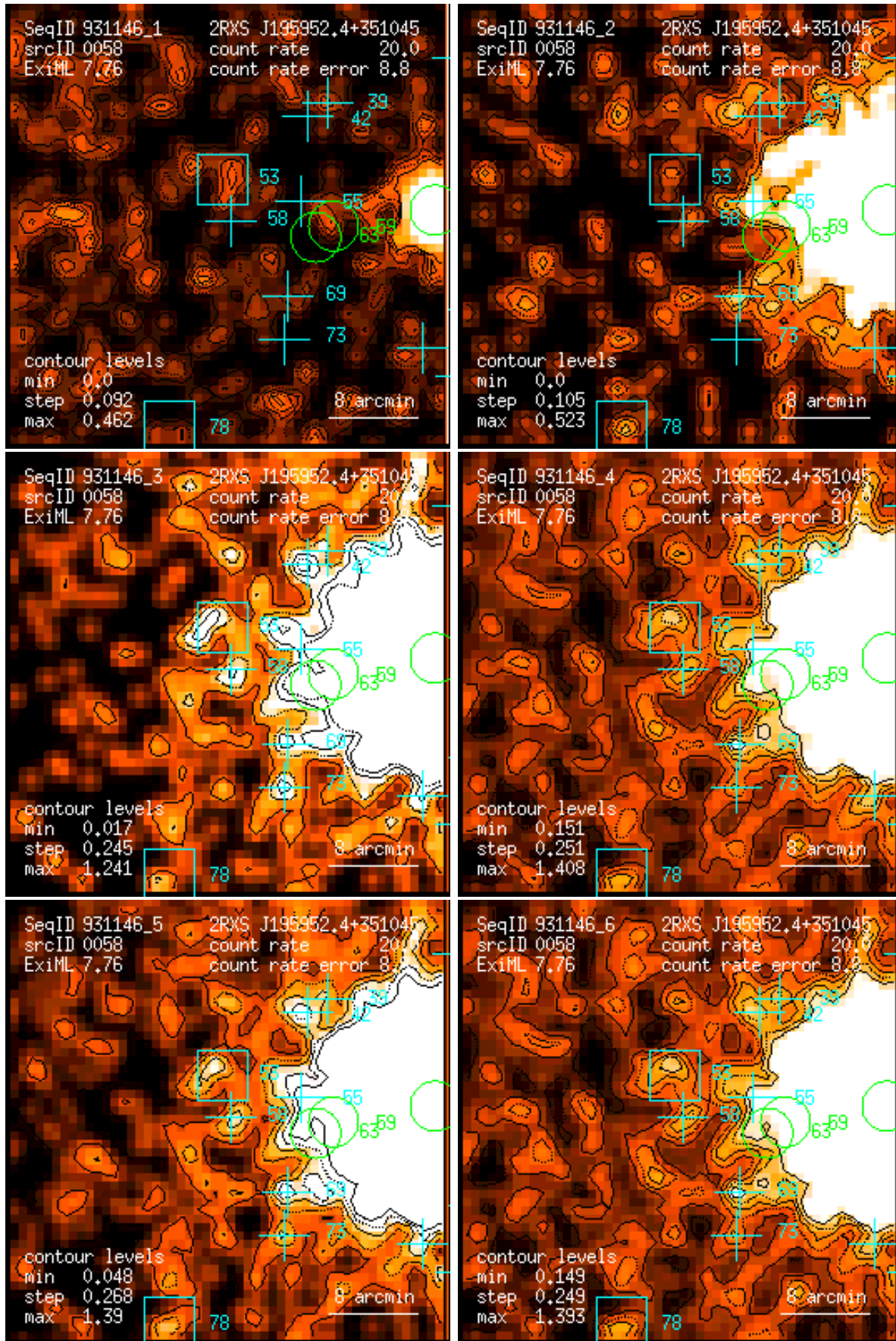
Figure 58: RASS 931146: detection 0058: band rate images, Gaussian filter: (1) PSPC channels 11 – 41, (2) 52 – 90, (3) 91 – 201, (4) 11 – 235, (5) 52 – 201, (6) 11 – 201. Broad band rates in counts/ks. Band rate contour levels in counts/ks/arcmin 2 .
