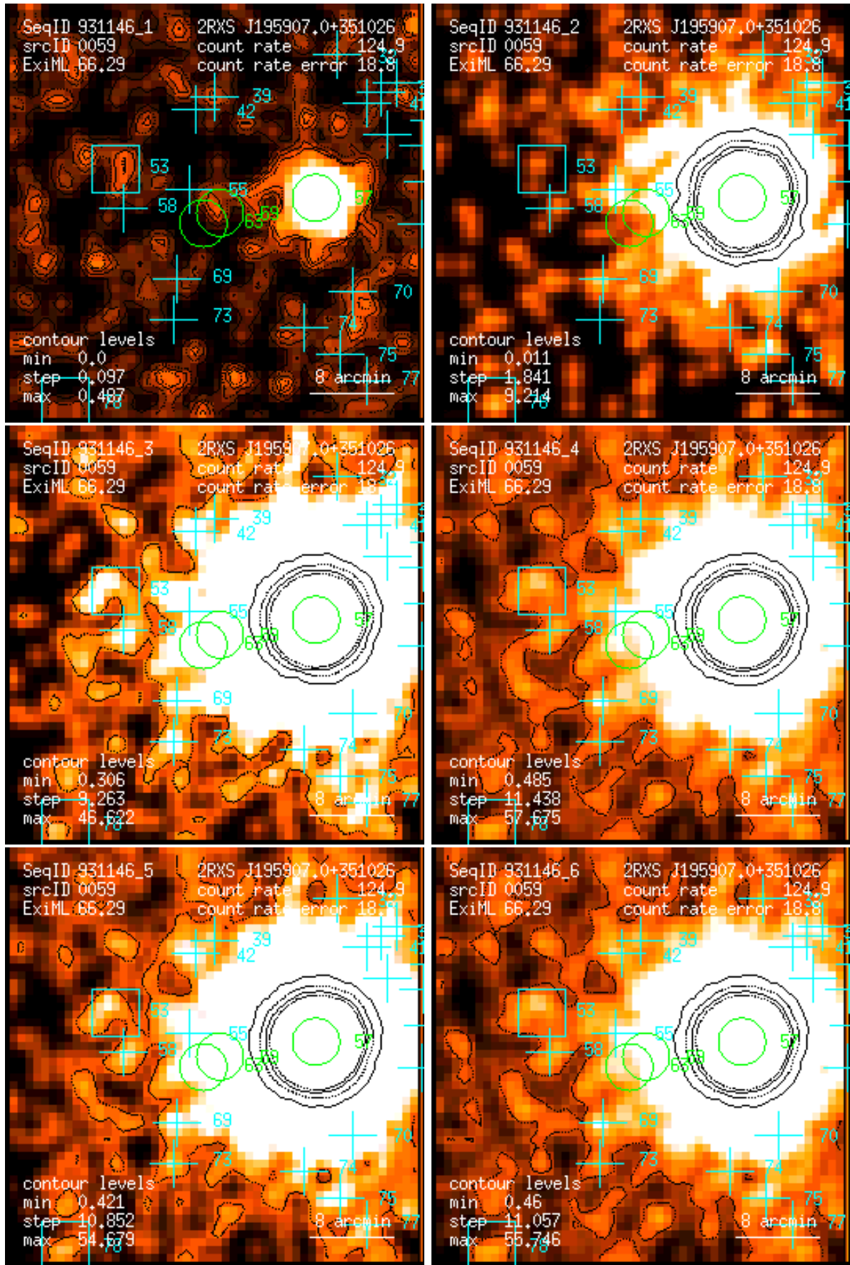
Figure 59: RASS 931146: detection 0059: band rate images, Gaussian filter: (1) PSPC channels 11 – 41, (2) 52 – 90, (3) 91 – 201, (4) 11 – 235, (5) 52 – 201, (6) 11 – 201. Broad band rates in counts/ks. Band rate contour levels in counts/ks/arcmin 2 .
