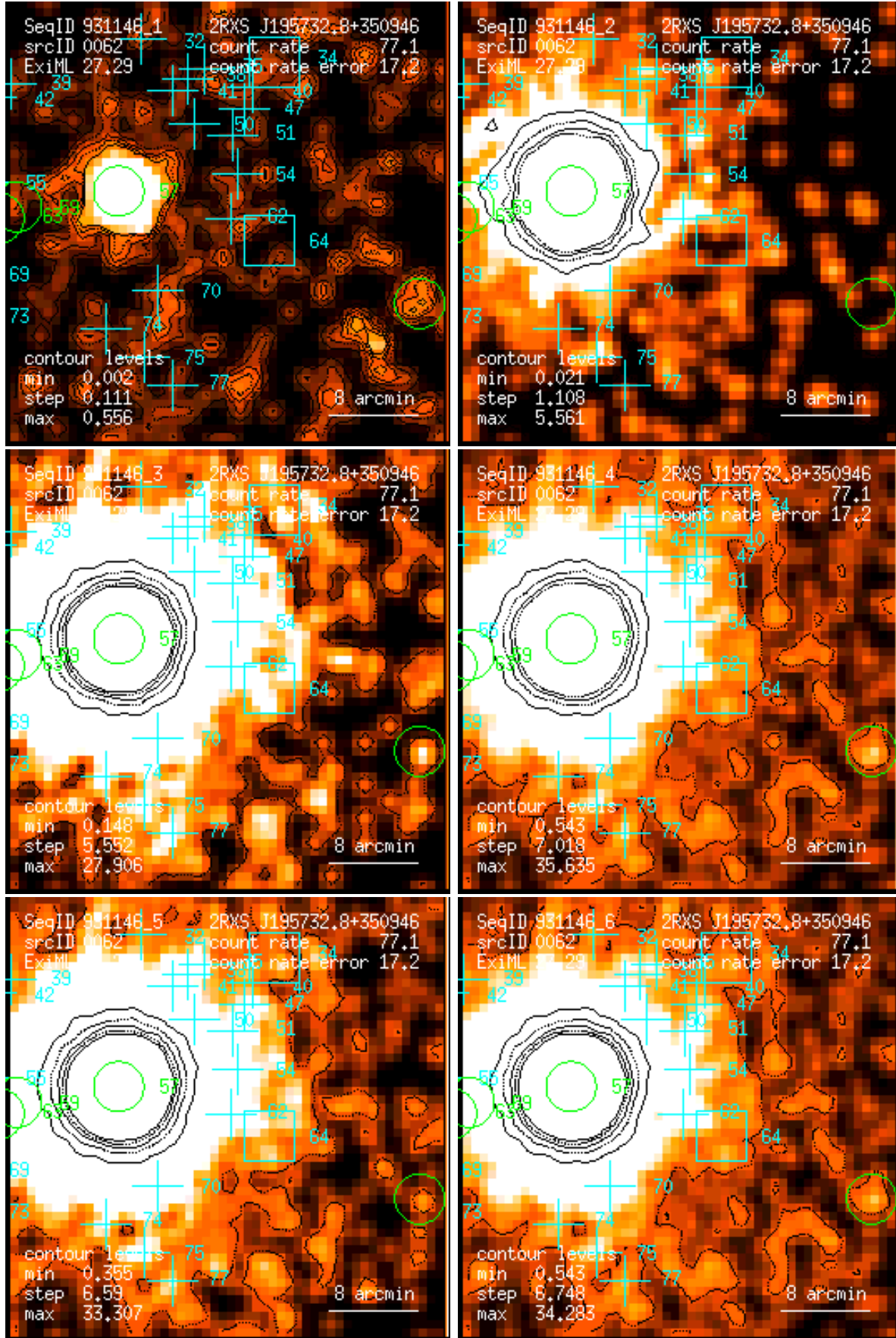
Figure 62: RASS 931146: detection 0062: band rate images, Gaussian filter: (1) PSPC channels 11 – 41, (2) 52 – 90, (3) 91 – 201, (4) 11 – 235, (5) 52 – 201, (6) 11 – 201. Broad band rates in counts/ks. Band rate contour levels in counts/ks/arcmin 2 .
