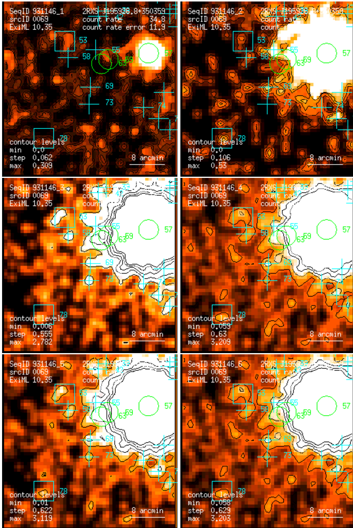
Figure 69: RASS 931146: detection 0069: band rate images, Gaussian filter: (1) PSPC channels 11 – 41, (2) 52 – 90, (3) 91 – 201, (4) 11 – 235, (5) 52 – 201, (6) 11 – 201. Broad band rates in counts/ks. Band rate contour levels in counts/ks/arcmin 2 .
