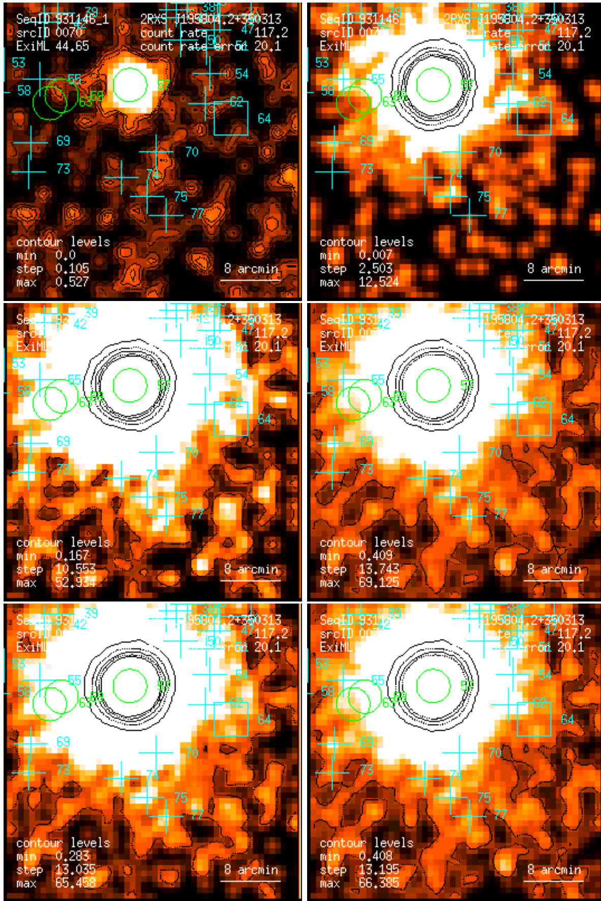
Figure 70: RASS 931146: detection 0070: band rate images, Gaussian filter: (1) PSPC channels 11 – 41, (2) 52 – 90, (3) 91 – 201, (4) 11 – 235, (5) 52 – 201, (6) 11 – 201. Broad band rates in counts/ks. Band rate contour levels in counts/ks/arcmin 2 .
