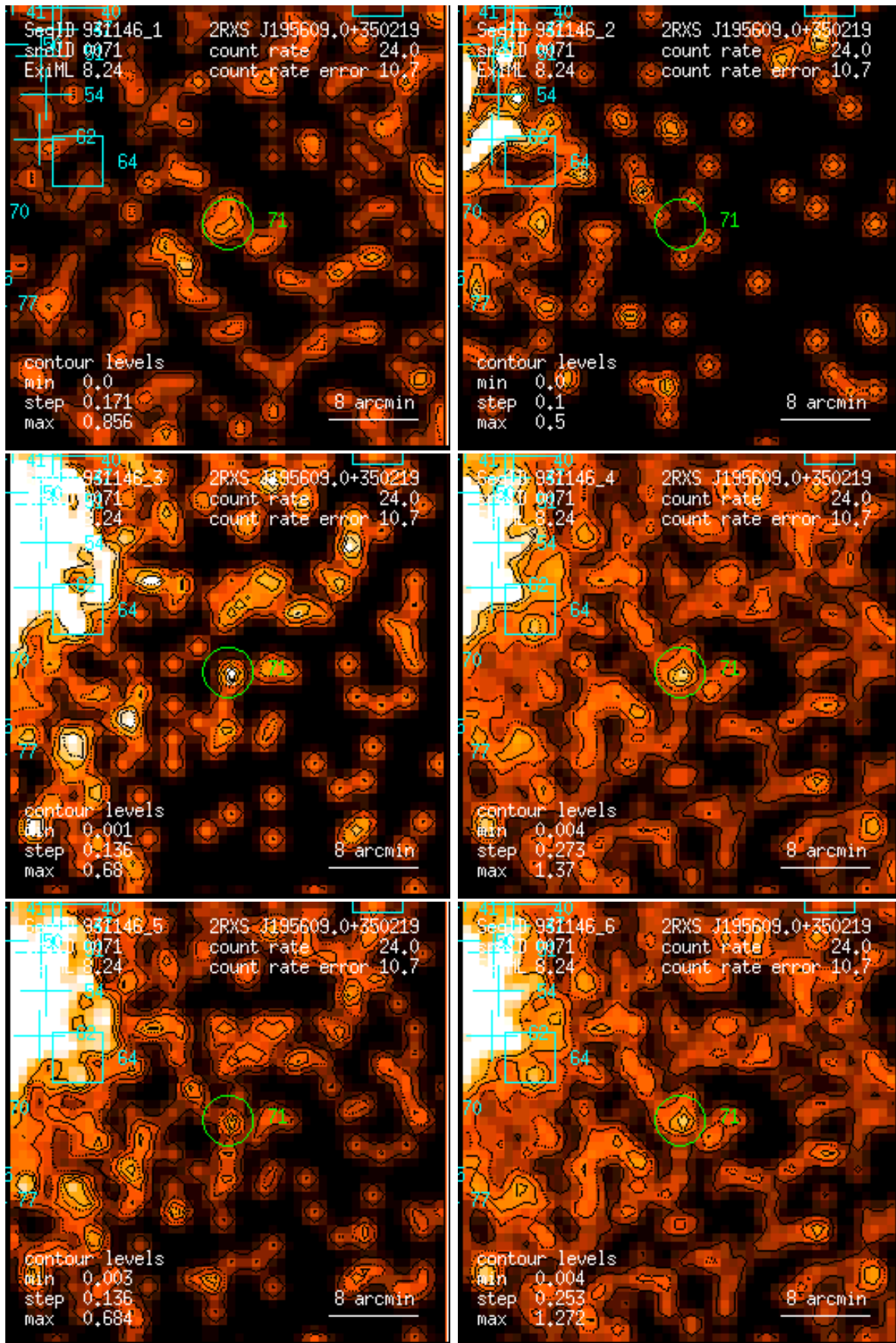
Figure 71: RASS 931146: detection 0071: band rate images, Gaussian filter: (1) PSPC channels 11 – 41, (2) 52 – 90, (3) 91 – 201, (4) 11 – 235, (5) 52 – 201, (6) 11 – 201. Broad band rates in counts/ks. Band rate contour levels in counts/ks/arcmin 2 .
