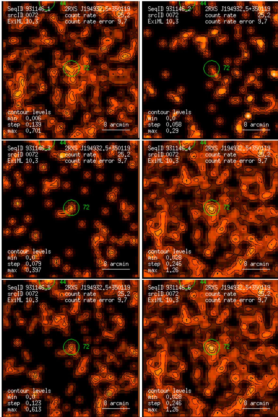
Figure 72: RASS 931146: detection 0072: band rate images, Gaussian filter: (1) PSPC channels 11 – 41, (2) 52 – 90, (3) 91 – 201, (4) 11 – 235, (5) 52 – 201, (6) 11 – 201. Broad band rates in counts/ks. Band rate contour levels in counts/ks/arcmin 2 .
