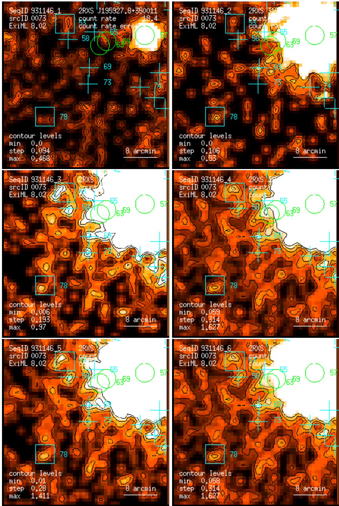
Figure 73: RASS 931146: detection 0073: band rate images, Gaussian filter: (1) PSPC channels 11 – 41, (2) 52 – 90, (3) 91 – 201, (4) 11 – 235, (5) 52 – 201, (6) 11 – 201. Broad band rates in counts/ks. Band rate contour levels in counts/ks/arcmin 2 .
