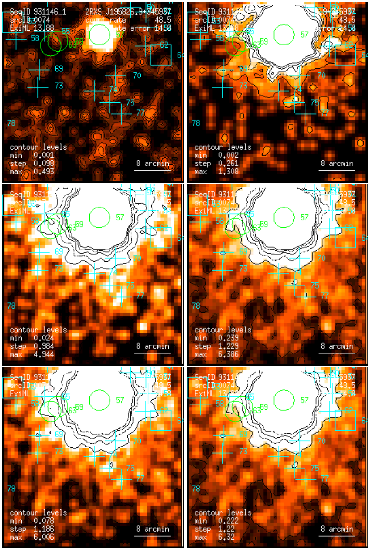
Figure 74: RASS 931146: detection 0074: band rate images, Gaussian filter: (1) PSPC channels 11 – 41, (2) 52 – 90, (3) 91 – 201, (4) 11 – 235, (5) 52 – 201, (6) 11 – 201. Broad band rates in counts/ks. Band rate contour levels in counts/ks/arcmin 2 .
