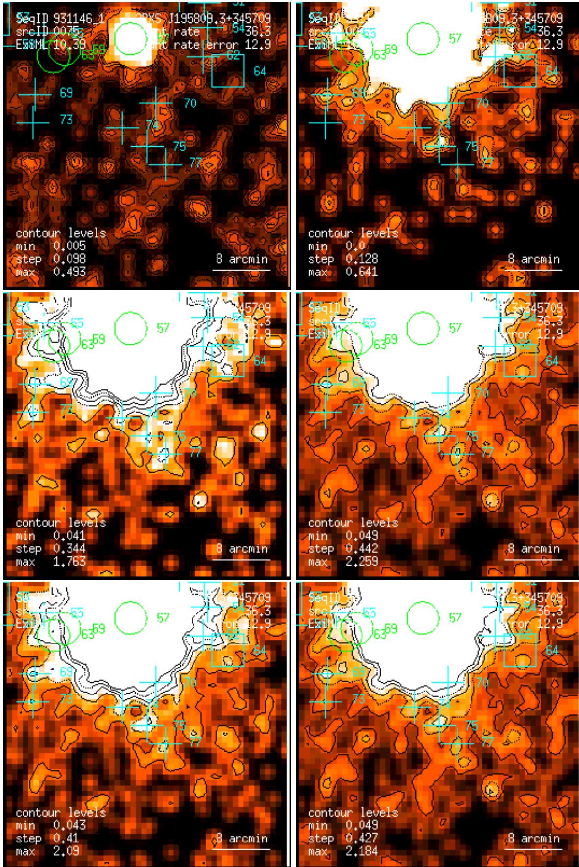
Figure 75: RASS 931146: detection 0075: band rate images, Gaussian filter: (1) PSPC channels 11 – 41, (2) 52 – 90, (3) 91 – 201, (4) 11 – 235, (5) 52 – 201, (6) 11 – 201. Broad band rates in counts/ks. Band rate contour levels in counts/ks/arcmin 2 .
