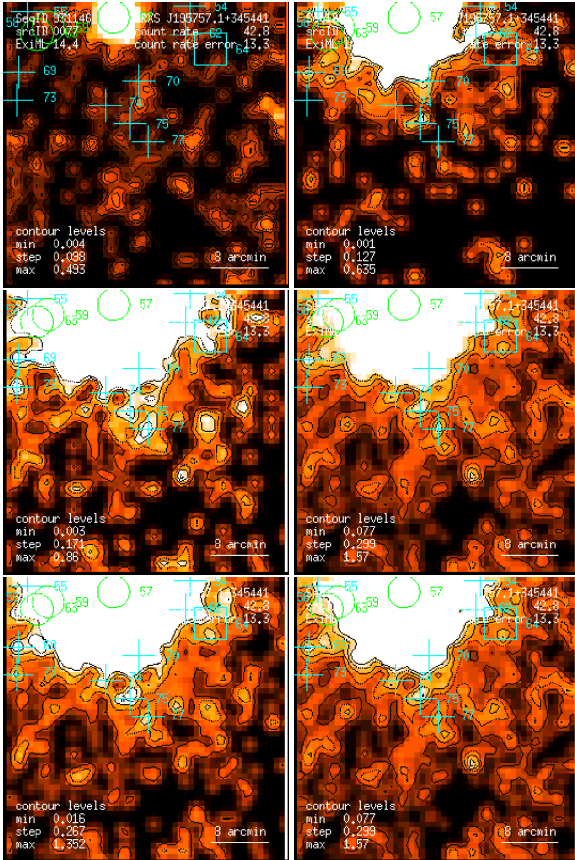
Figure 77: RASS 931146: detection 0077: band rate images, Gaussian filter: (1) PSPC channels 11 – 41, (2) 52 – 90, (3) 91 – 201, (4) 11 – 235, (5) 52 – 201, (6) 11 – 201. Broad band rates in counts/ks. Band rate contour levels in counts/ks/arcmin 2 .
