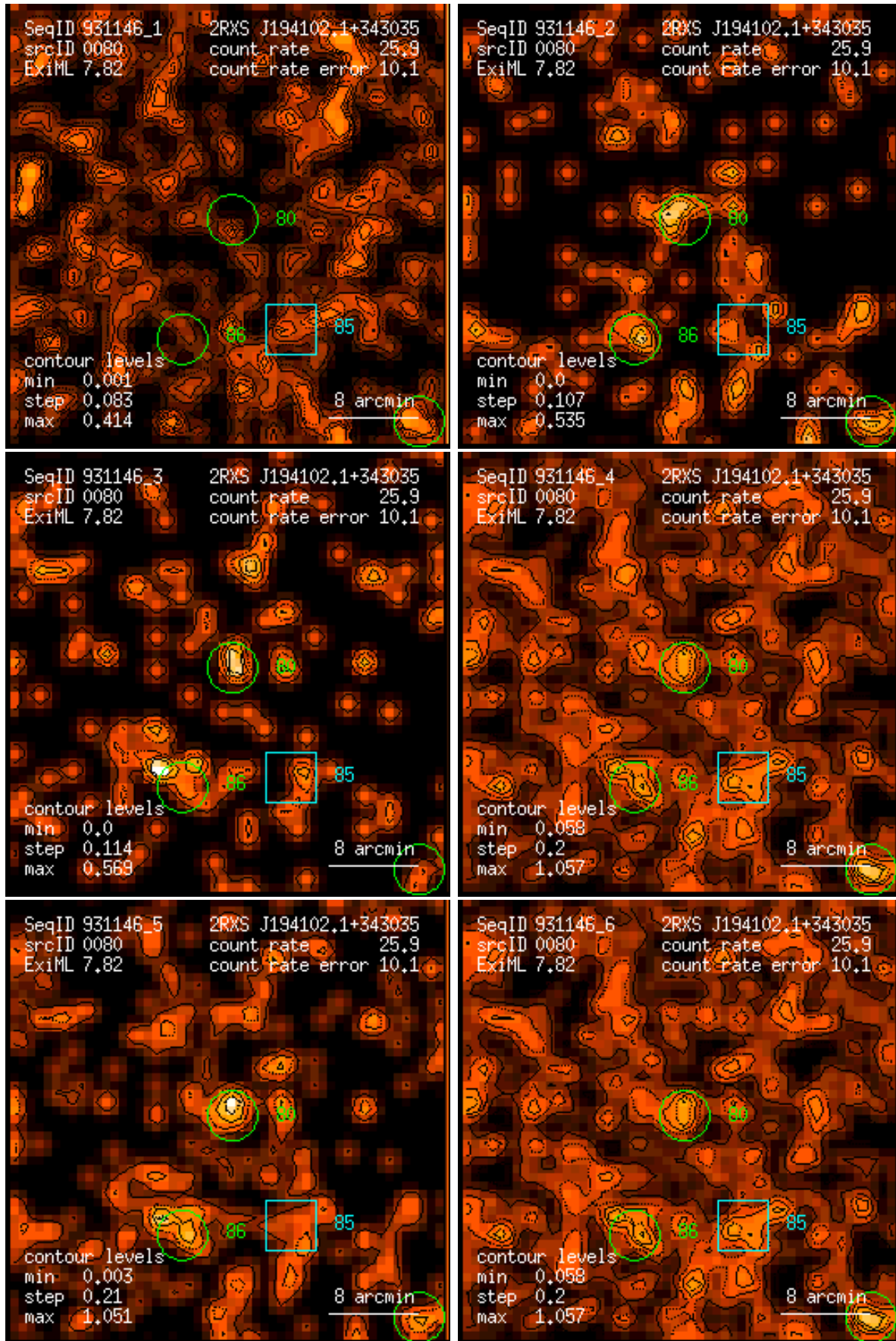
Figure 80: RASS 931146: detection 0080: band rate images, Gaussian filter: (1) PSPC channels 11 – 41, (2) 52 – 90, (3) 91 – 201, (4) 11 – 235, (5) 52 – 201, (6) 11 – 201. Broad band rates in counts/ks. Band rate contour levels in counts/ks/arcmin 2 .
