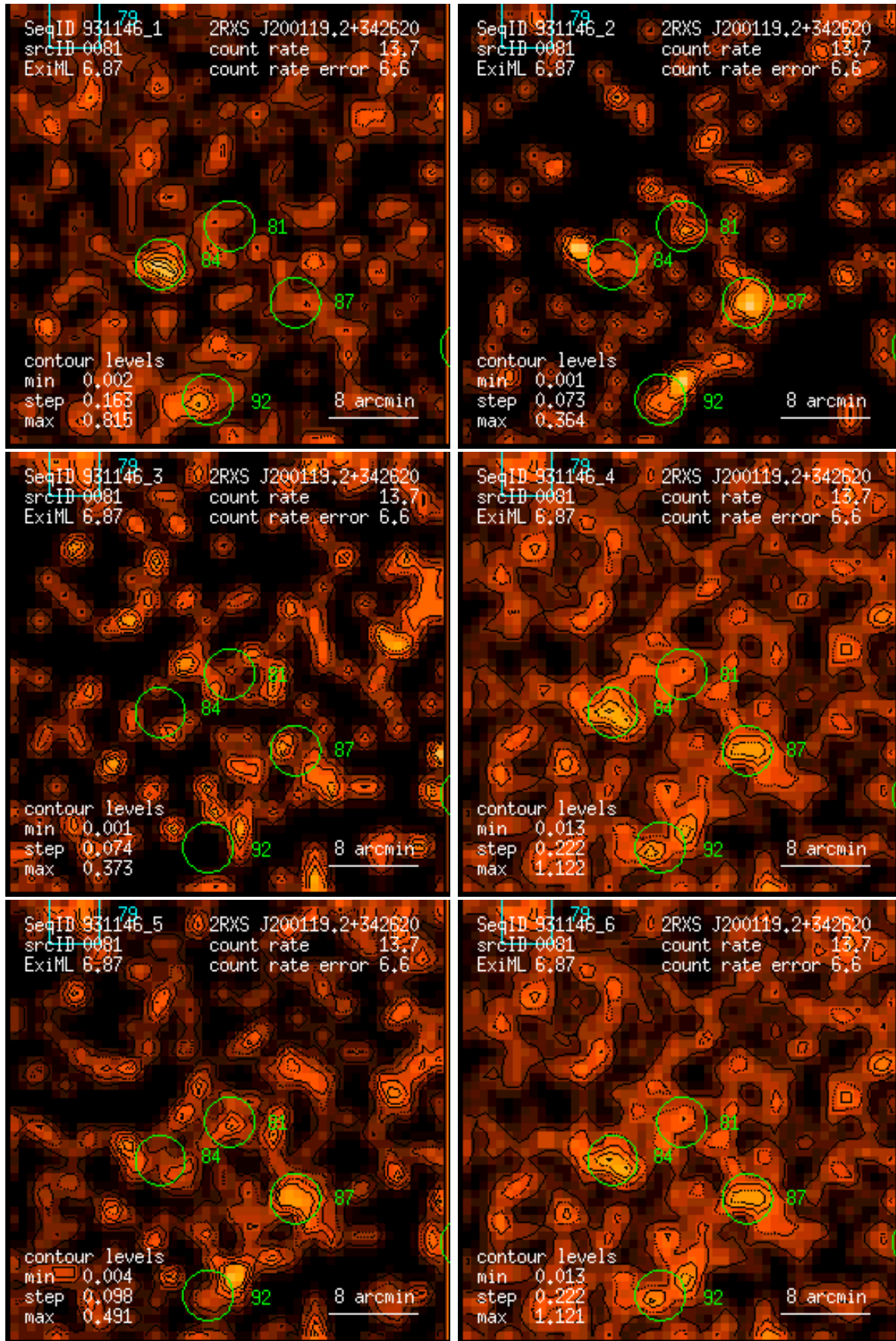
Figure 81: RASS 931146: detection 0081: band rate images, Gaussian filter: (1) PSPC channels 11 – 41, (2) 52 – 90, (3) 91 – 201, (4) 11 – 235, (5) 52 – 201, (6) 11 – 201. Broad band rates in counts/ks. Band rate contour levels in counts/ks/arcmin 2 .
